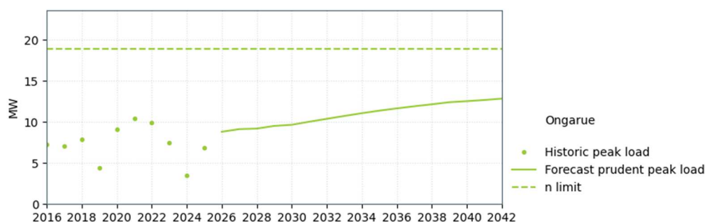
Figure 11-13: Ongarue supply capacity
