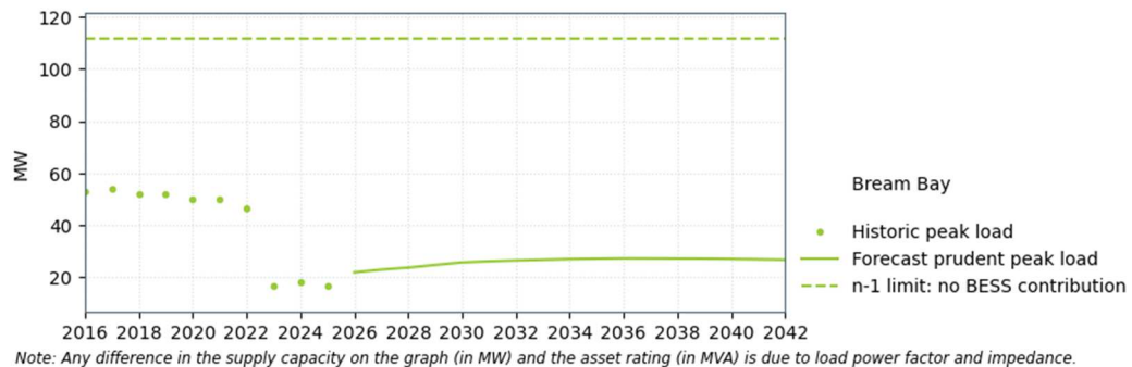
Figure 7-4: Bream Bay supply capacity
