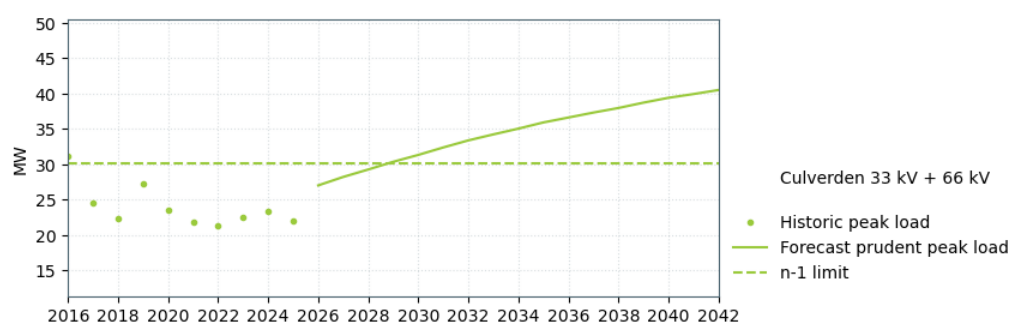
Figure 17-12: Culverden 220/33 kV supply capacity (combined 33 kV and 66 kV load)
