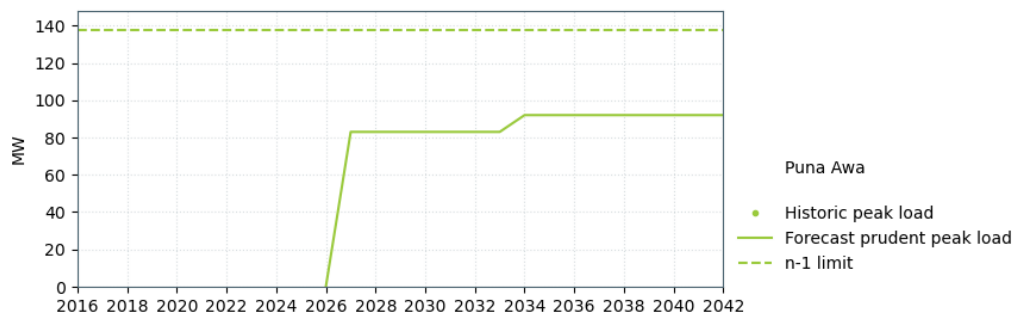
Figure 19-11: New Puna Awa GXP supply capacity
