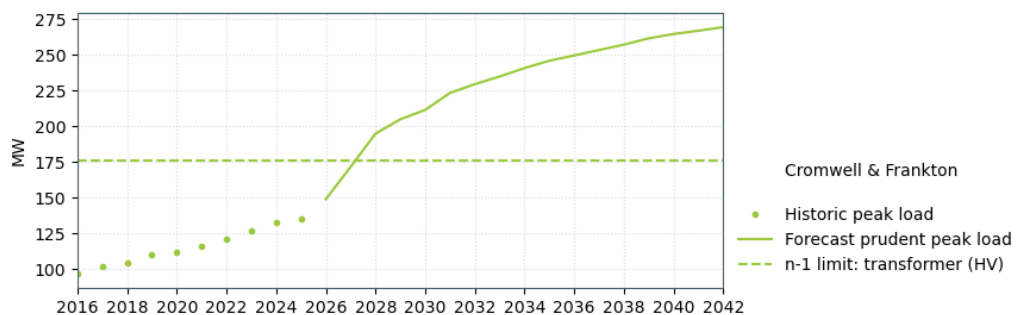
Figure 19-4: Cromwell (220 kV windings) supply capacity
