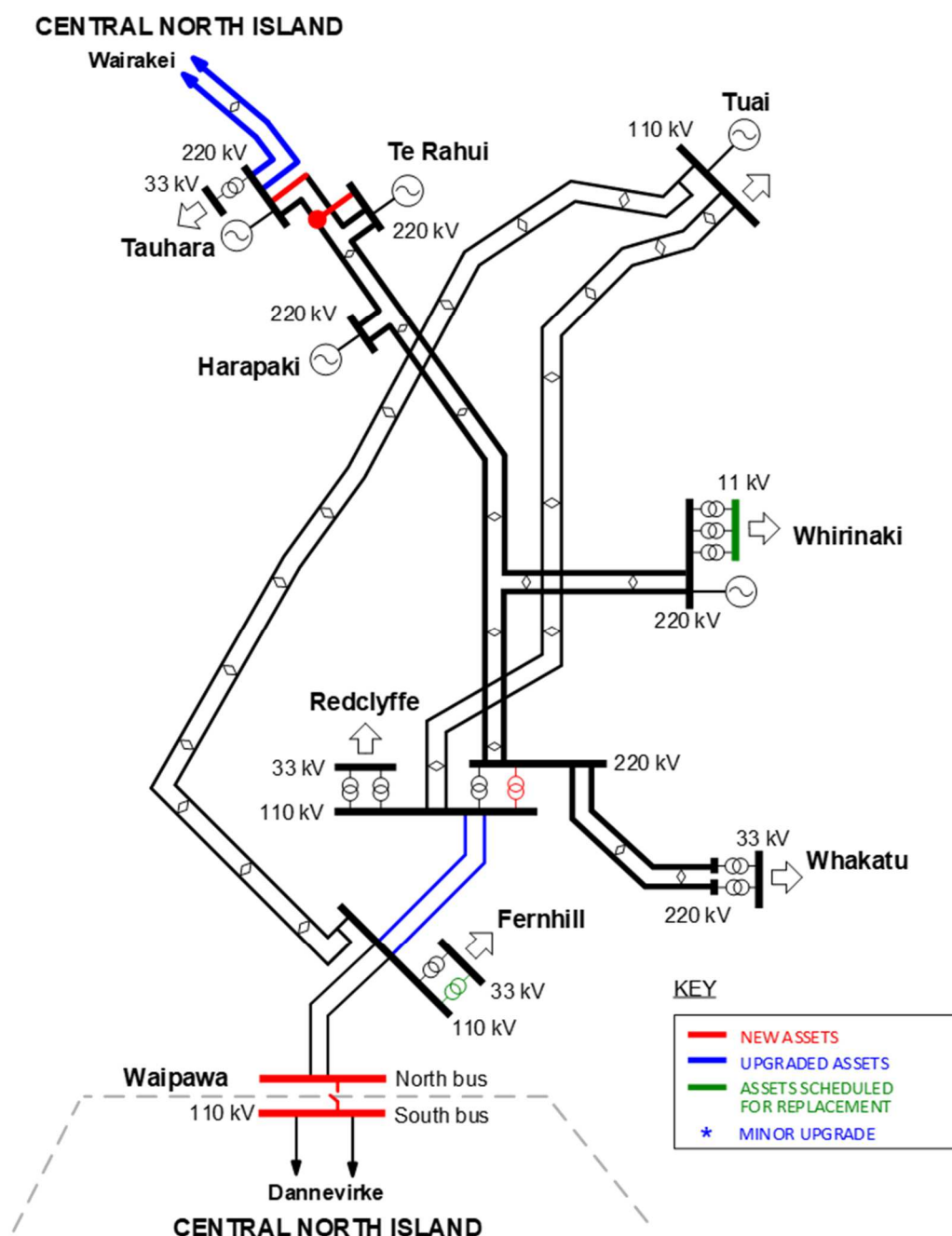
Figure 13-3: Possible Hawke's Bay transmission configuration in 2041
