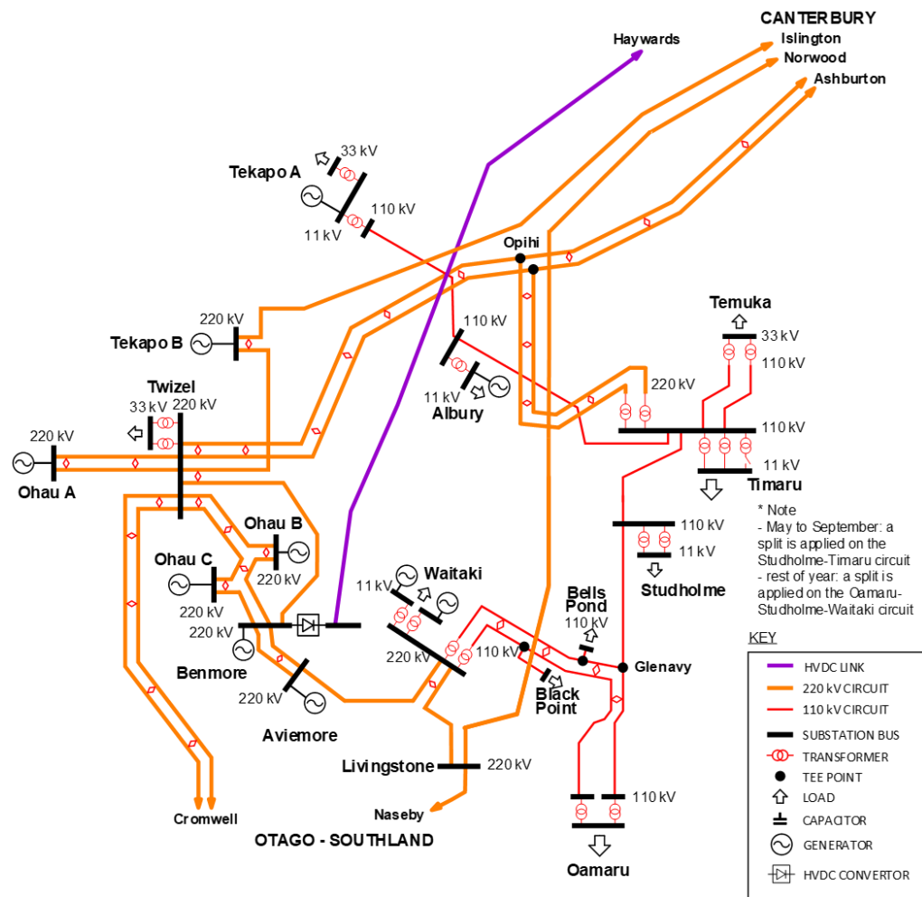
Figure 18-2: South Canterbury region transmission schematic
