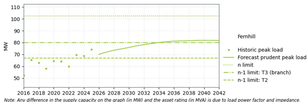
Figure 13-7: Fernhill supply capacity
