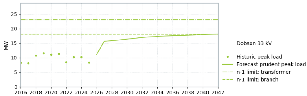
Figure 16-6: Dobson supply capacity
