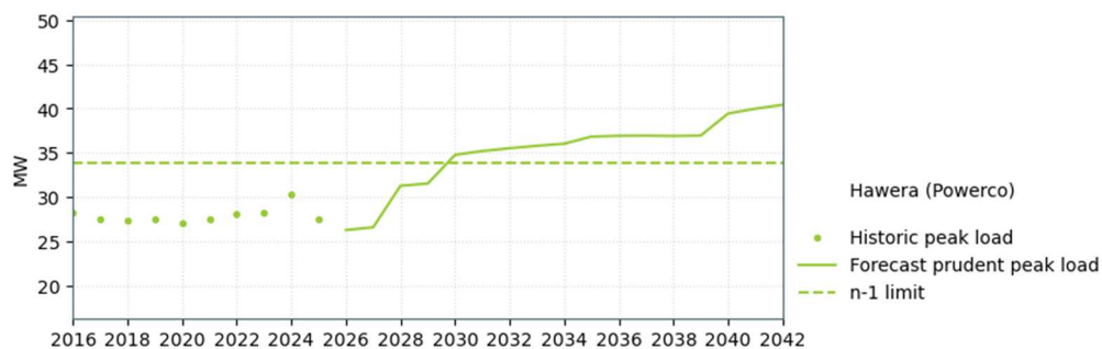
Figure 12-7: Hawera (Powerco) supply capacity
