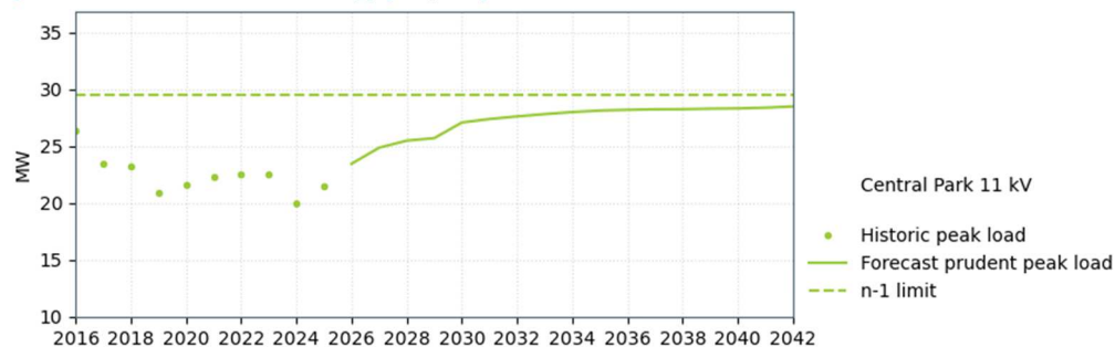
Figure 14-6: Central Park 11 kV supply capacity
