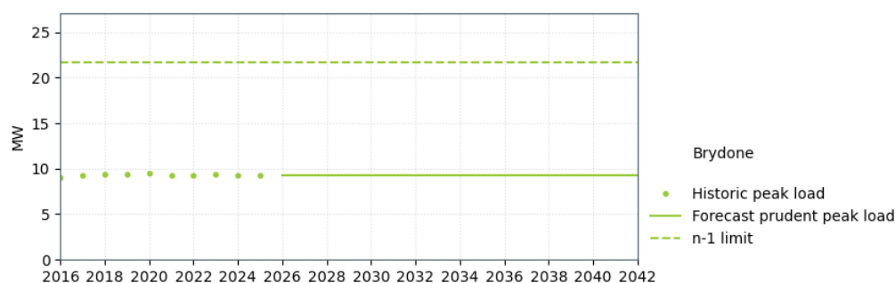
Figure 19-7: Brydone supply capacity
