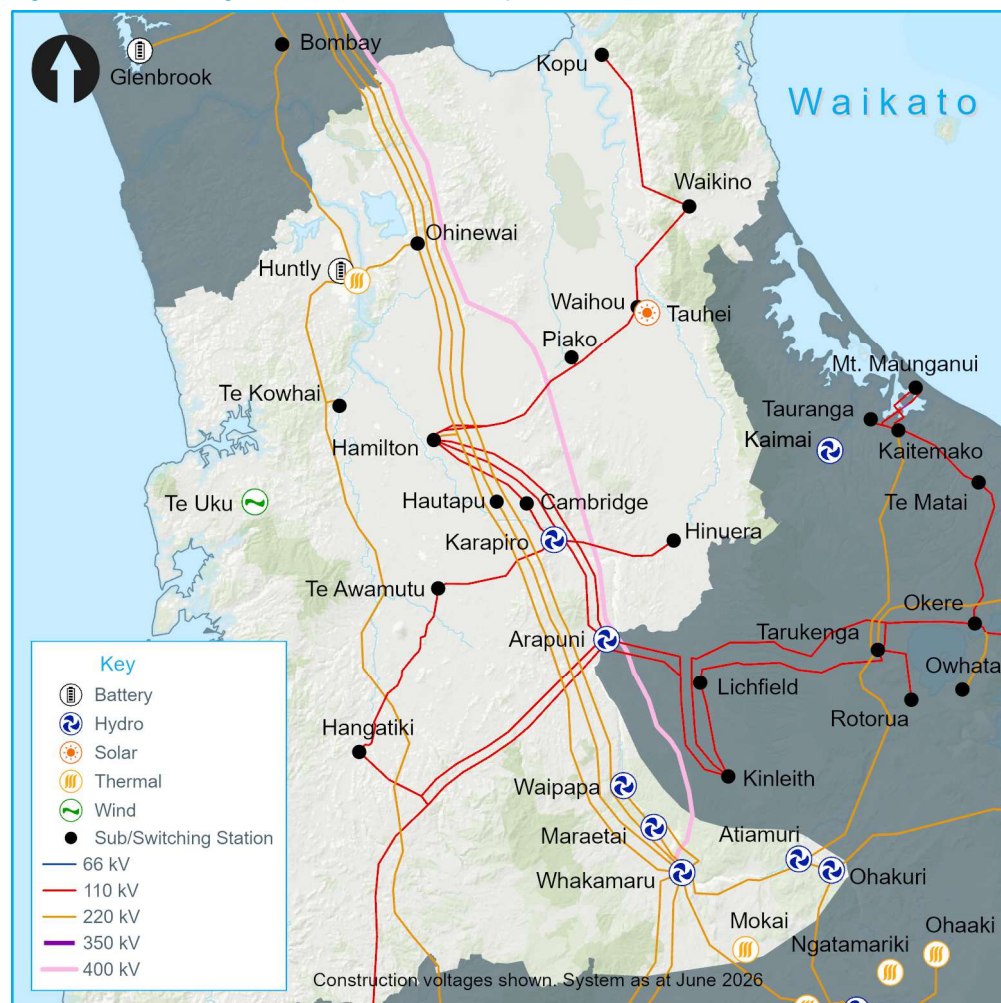
Figure 9-1: Waikato region transmission network map
