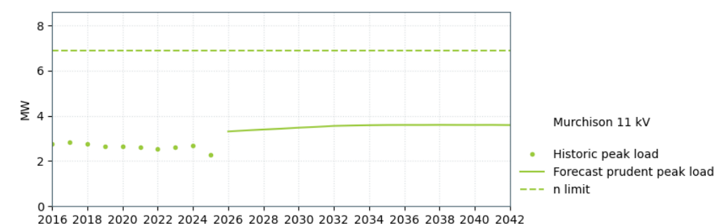
Figure 16-10: Murchison supply capacity
