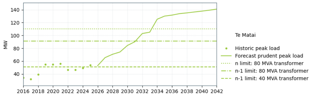
Figure 10-23: Te Matai supply capacity and supply limits (before T1 replacement)
