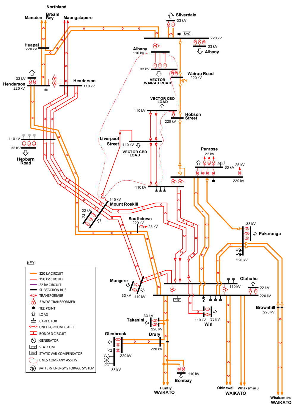
Figure 8-2: Auckland region transmission schematic
