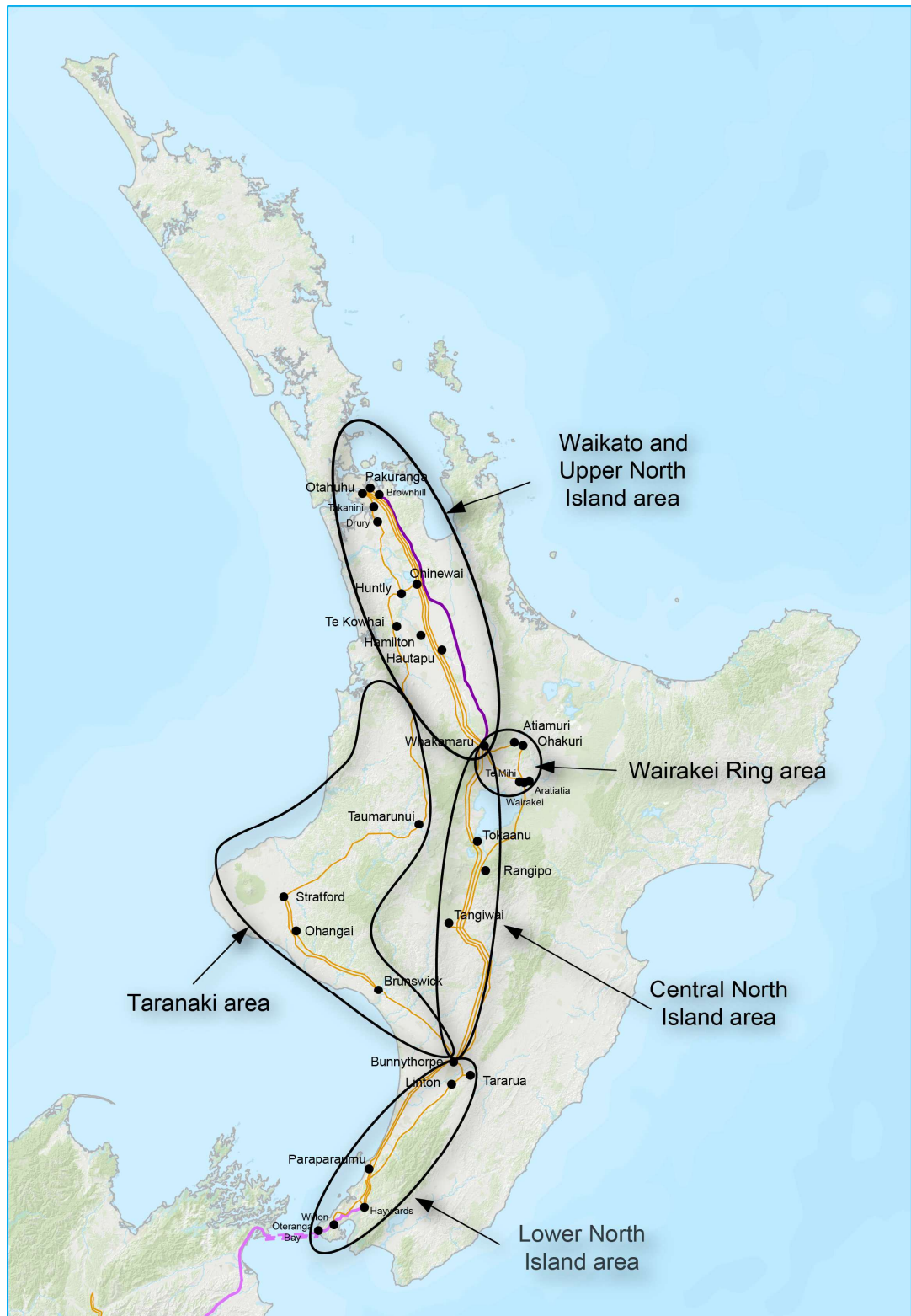
Figure 6-1: North Island grid backbone map
