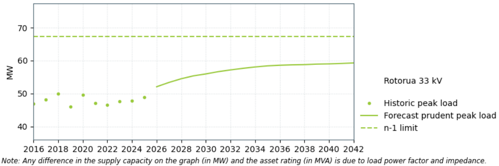
Figure 10-17: Rotorua 110/33 kV supply capacity
