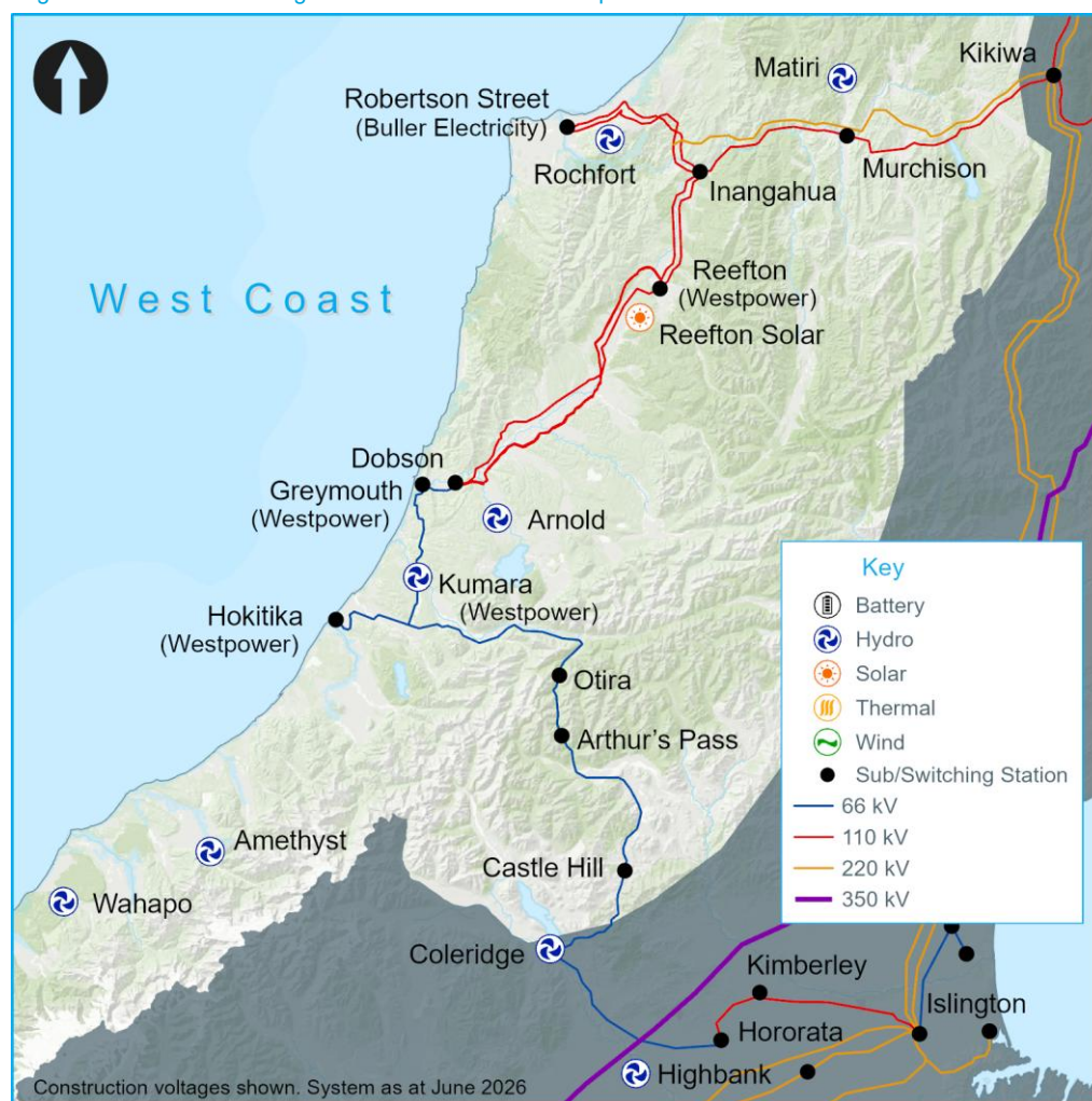
Figure 16-1: West Coast region transmission network map
