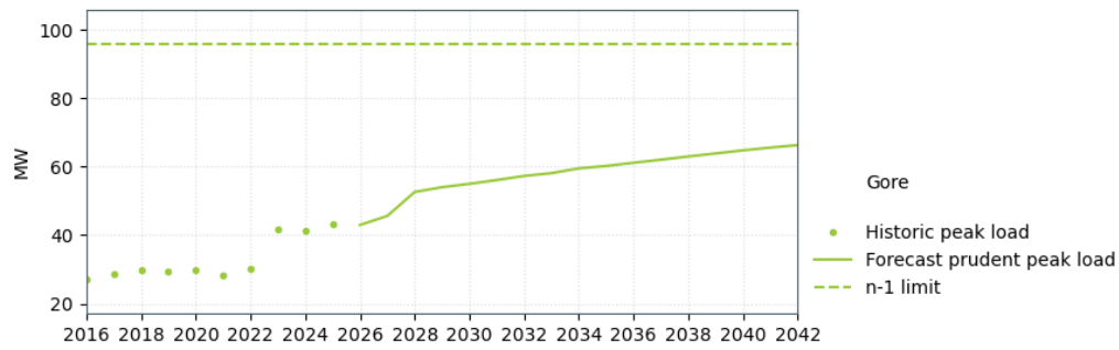
Figure 19-13: Gore supply capacity
