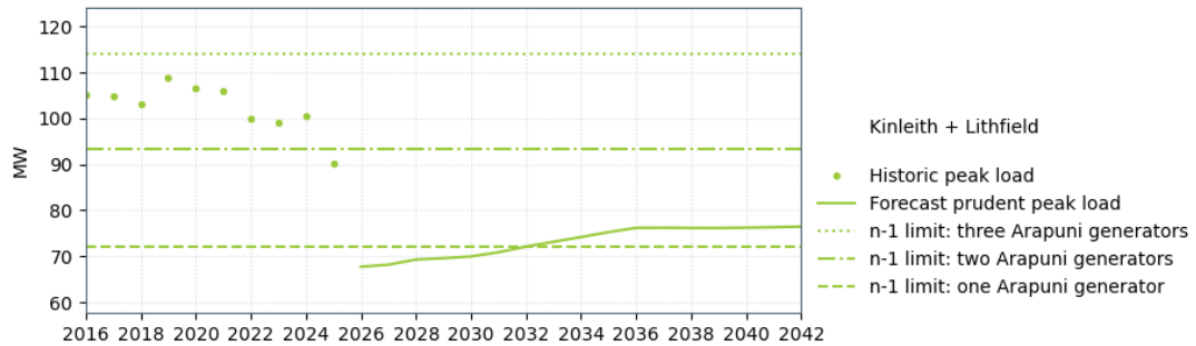
Figure 10-9: Lichfield–Tarukenga transmission capacity 12
