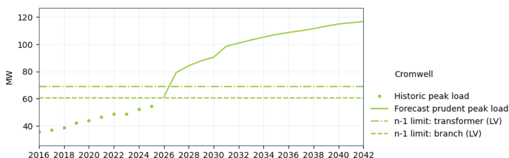
Figure 19-9: Cromwell (33 kV windings) supply capacity
