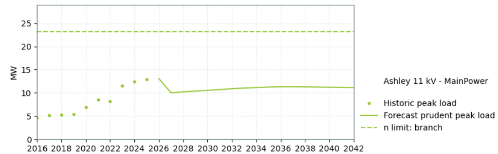
Figure 17-6: Ashley 11 kV supply capacity – MainPower
