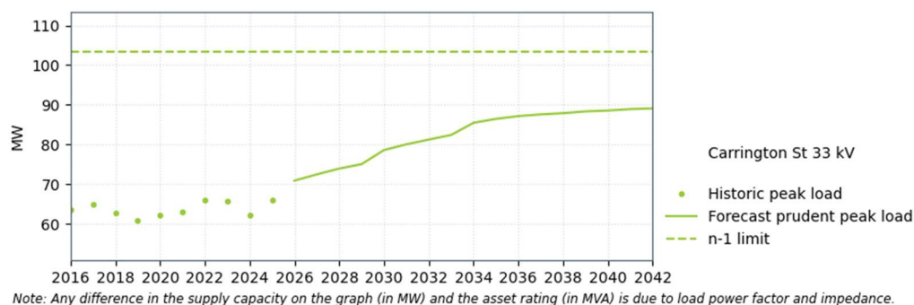
Figure 12-5: Carrington Street supply capacity
