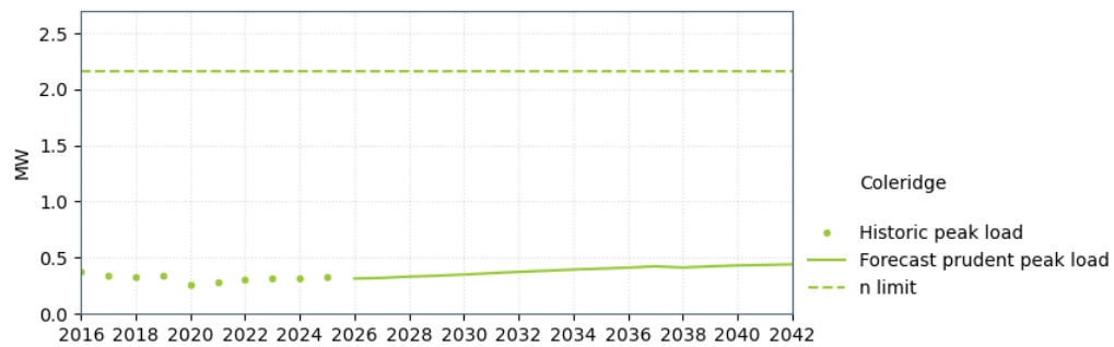
Figure 17-11: Coleridge supply capacity
