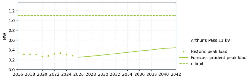
Figure 16-4: Arthur's Pass supply capacity
