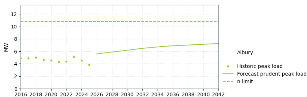
Figure 18-5: Albury supply capacity
