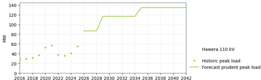
Figure 12-8: Hawera (Whareroa) supply capacity
