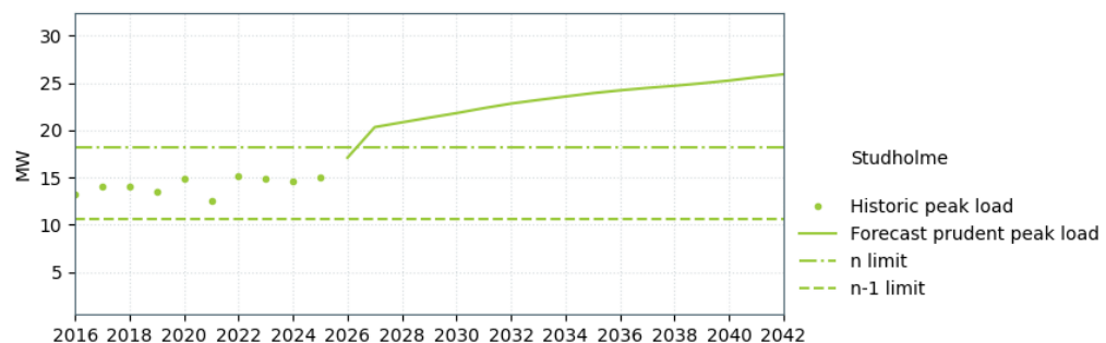
Figure 18-9: Studholme supply capacity
