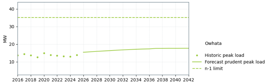
Figure 10-16: Owhata supply capacity
