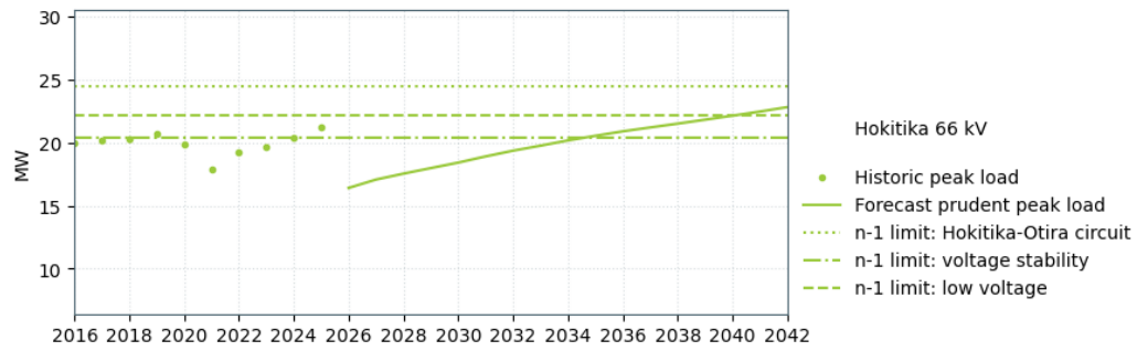
Figure 16-8: Hokitika–Otira transmission capacity
