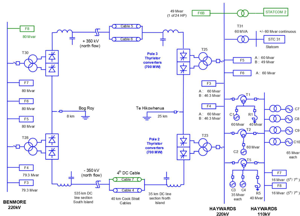
Figure 6-17: Simplified schematic of the existing HVDC link and possible configuration by 2041
