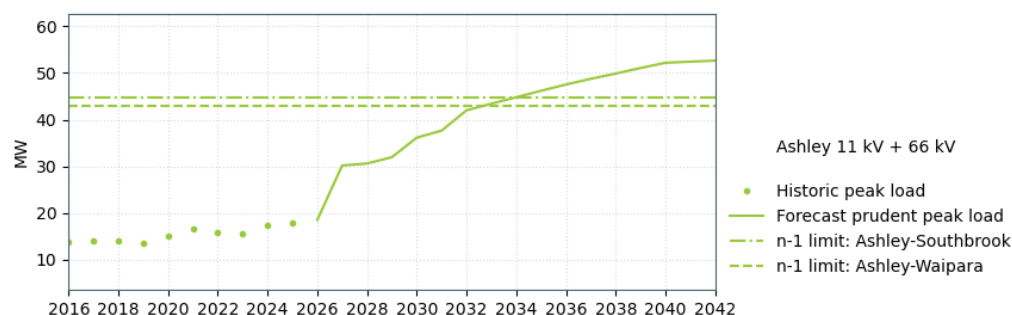
Figure 17-9: Ashley 11 kV and 66 kV supply capacity
