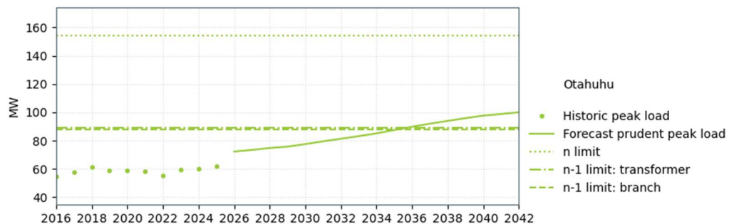
Figure 8-15: Otahuhu supply capacity
