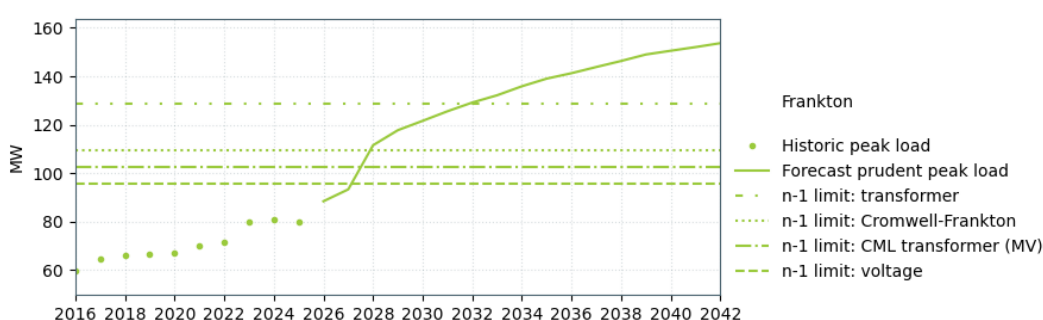
Figure 19-12: Frankton supply capacity
