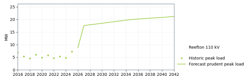
Figure 16-12: Reefton load forecast
