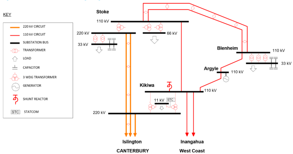
Figure 15-2: Nelson-Marlborough region transmission schematic
