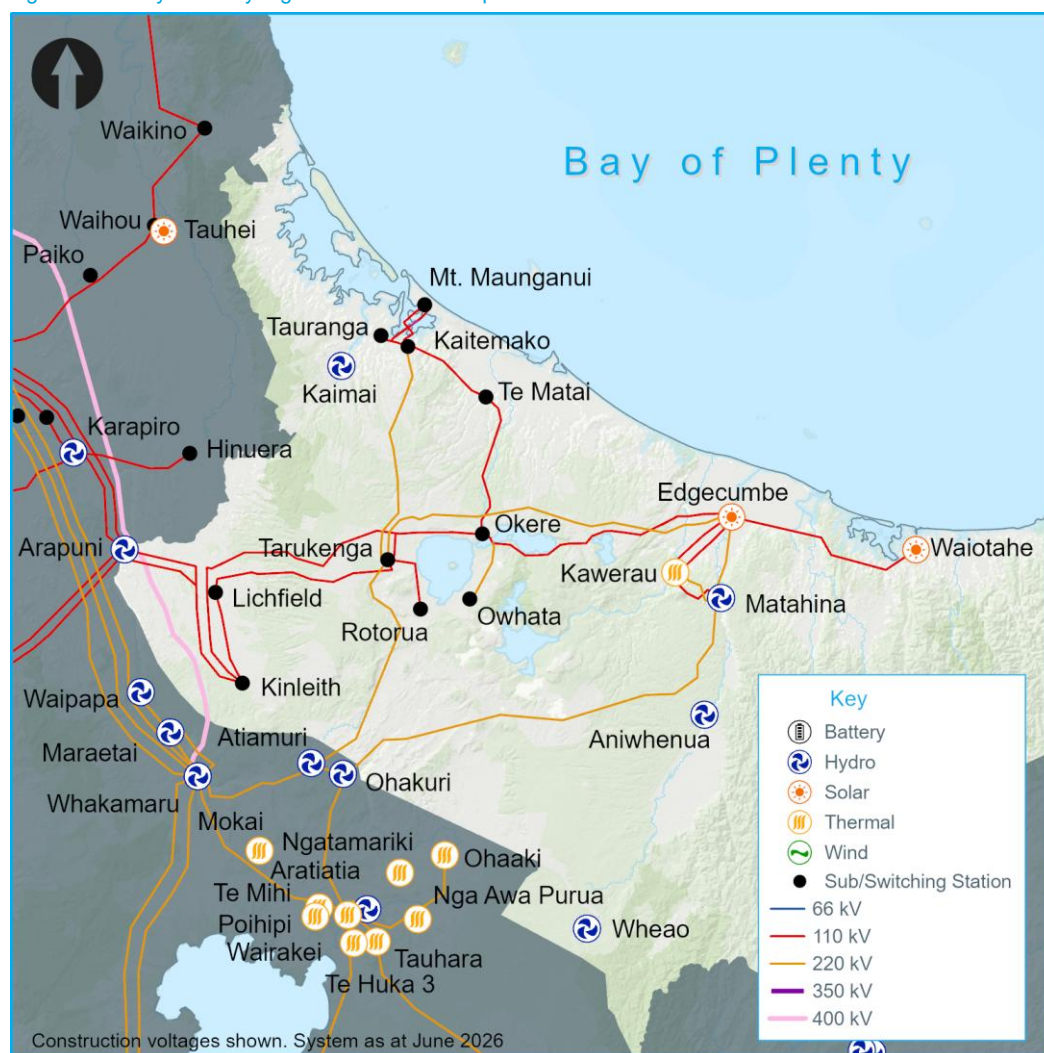
Figure 10-1: Bay of Plenty region transmission map
