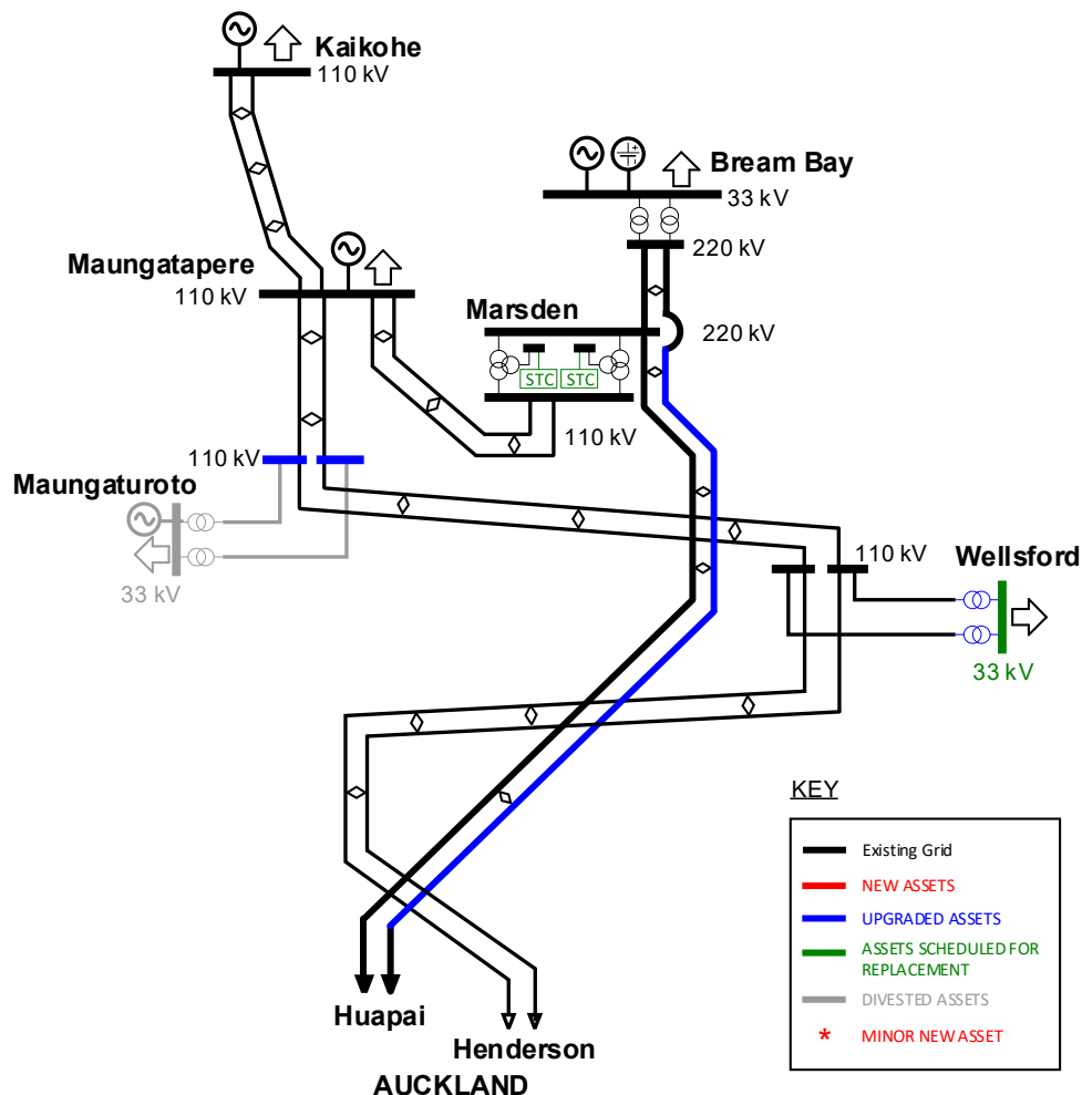
Figure 7-3: Possible Northland transmission configuration in 2041
