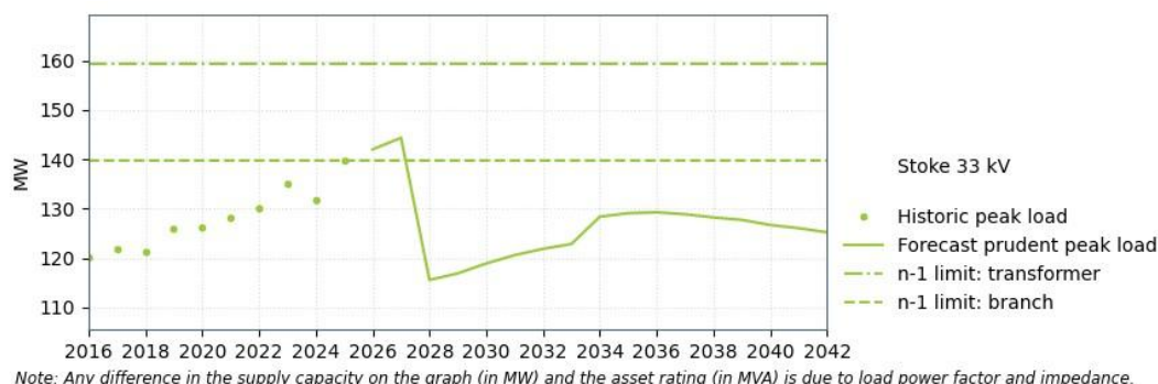
Figure 15-7: Stoke 33 kV supply capacity
