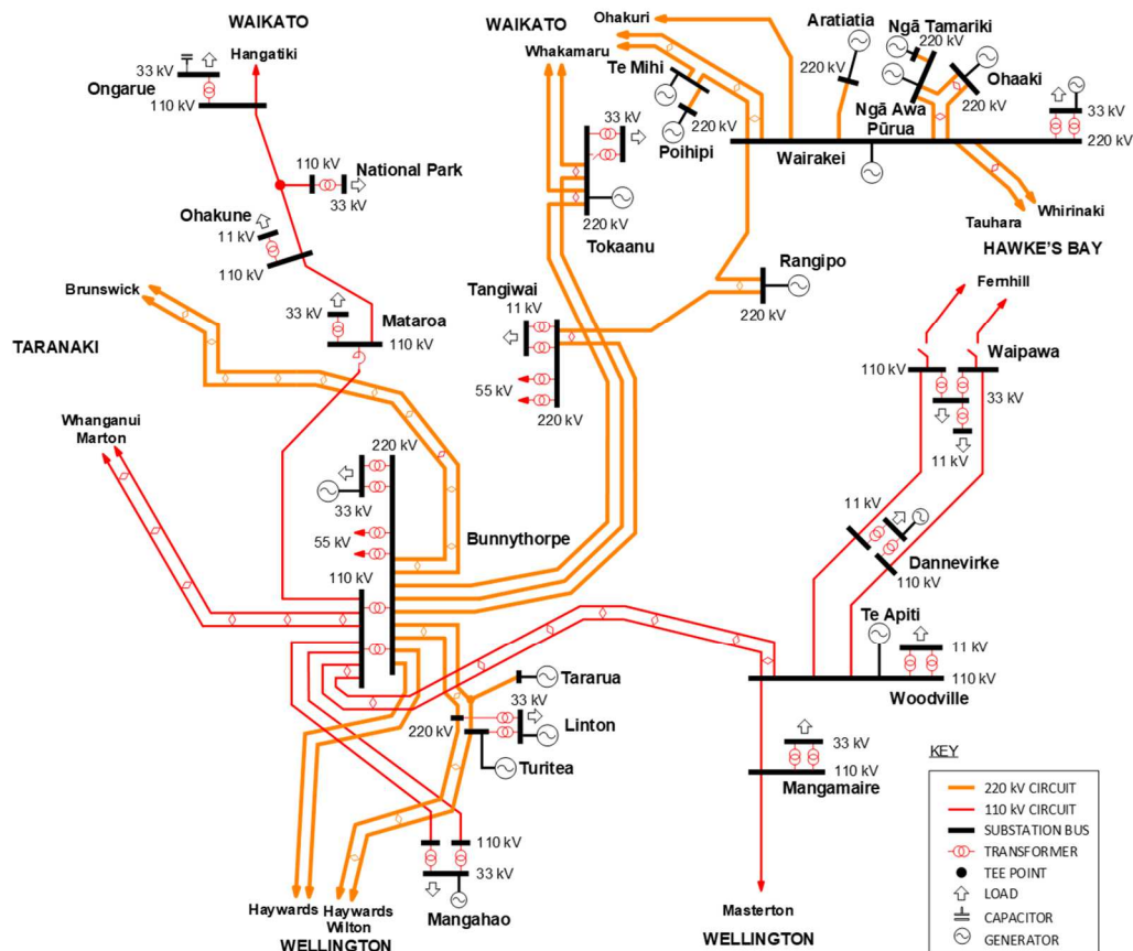
Figure 11-2: Central North Island region transmission schematic
