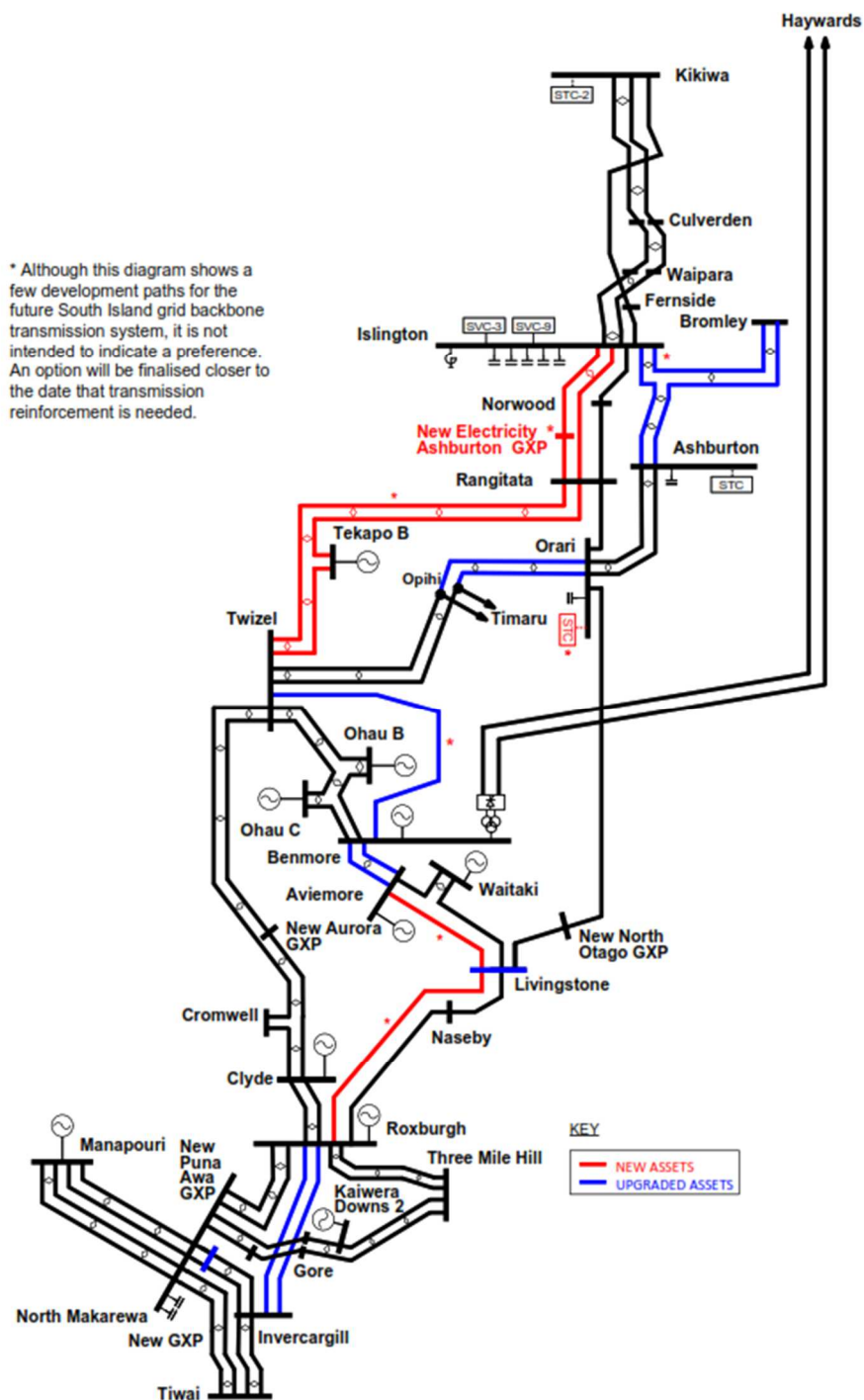
Figure 6-13: Longer-term indicative South Island grid backbone schematic (beyond 2041)
