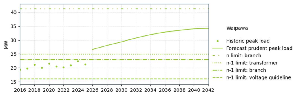
Figure 11-15: Waipawa 110/33 kV supply capacity
