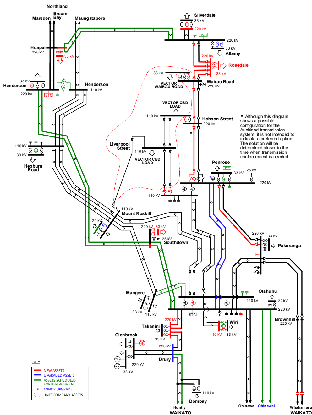
Figure 8-3: Possible Auckland transmission configuration in 2041
