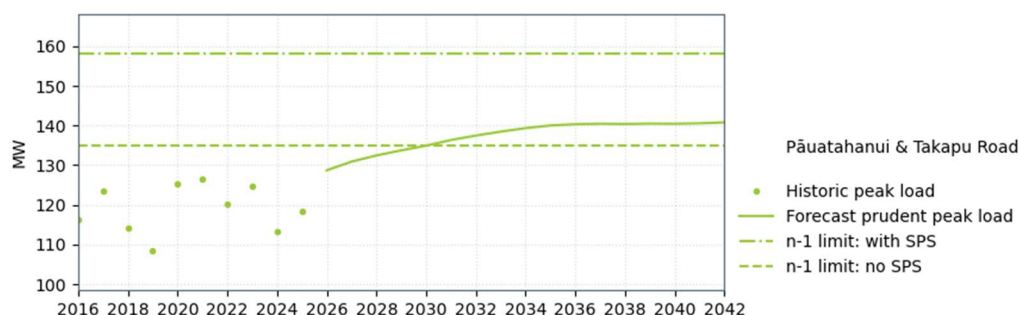
Figure 14-4: Combined Pāuatahanui and Takapu Road supply capacity
