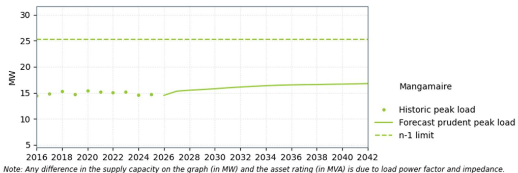
Figure 11-9: Mangamaire supply capacity
