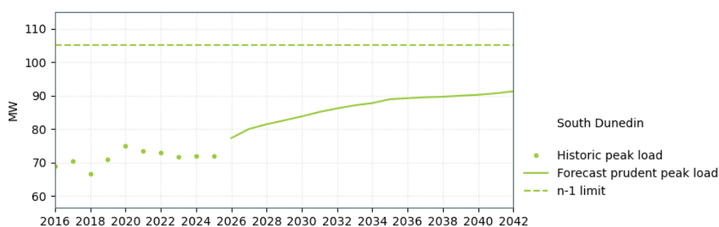
Figure 19-19: South Dunedin supply capacity
