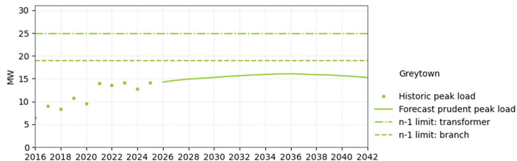
Figure 14-8: Greytown supply capacity
