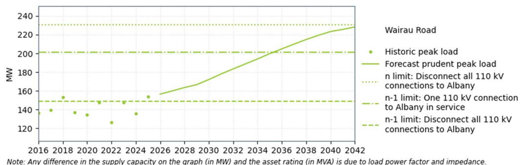
Figure 8-21: Wairau Road supply capacity
