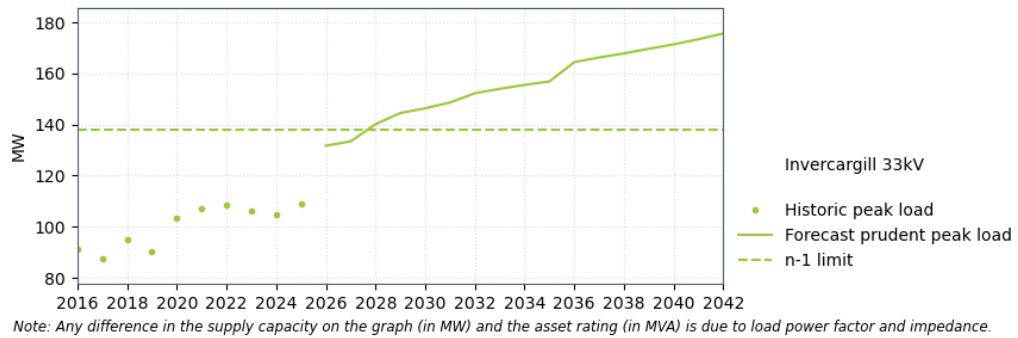
Figure 19-15: Invercargill 33 kV supply capacity
