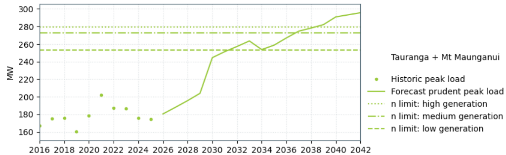
Figure 10-6: Kaitemako–Tauranga and Mount Maunganui transmission capacity low (14 MW), medium (33 MW), and high (40 MW) Kaimai generation levels
