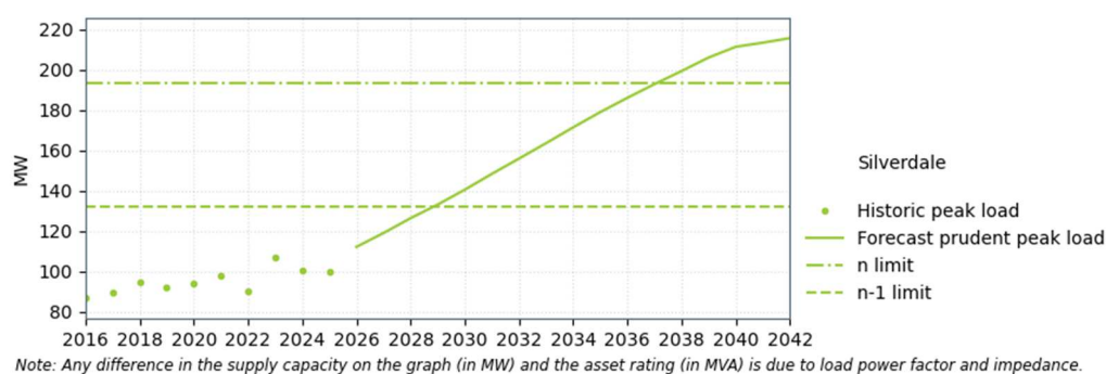
Figure 8-19: Silverdale supply capacity
