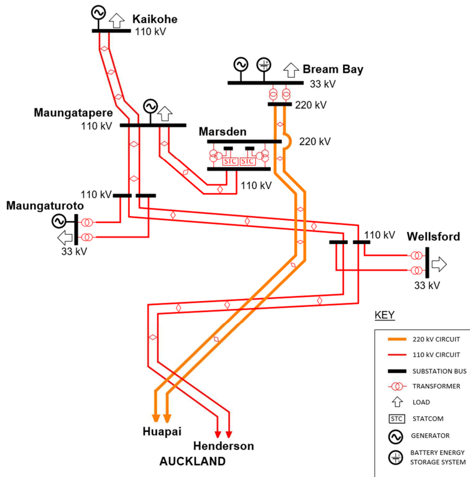
Figure 7-2: Northland region transmission schematic
