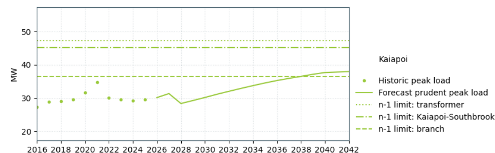
Figure 17-18: Kaiapoi supply capacity
