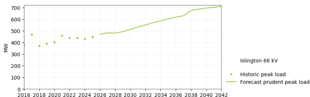
Figure 17-17: Islington 66 kV load forecast
