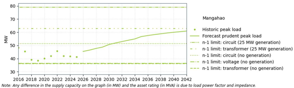
Figure 11-8: Mangahao supply capacity
