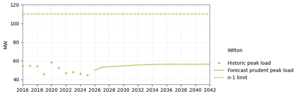
Figure 14-19: Wilton supply capacity
