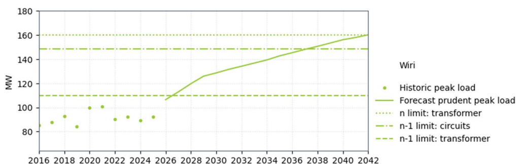
Figure 8-22: Wiri supply capacity
