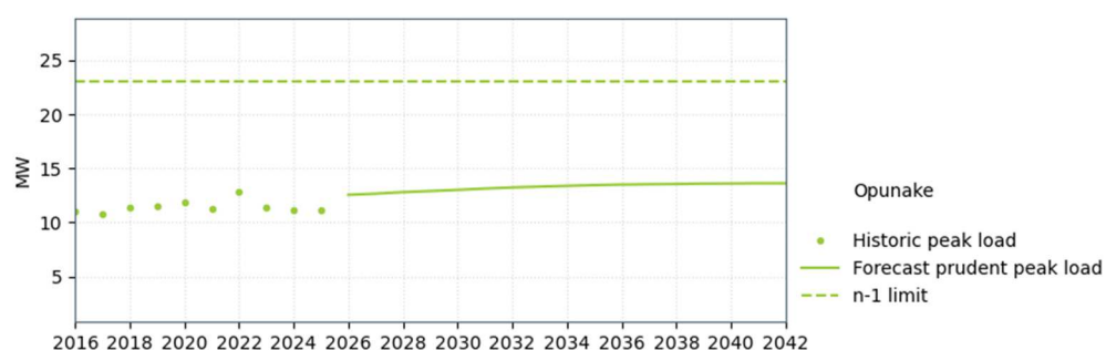
Figure 12-13: Opunake supply capacity
