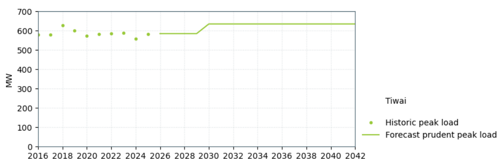
Figure 19-20: Tiwai 220 kV load forecast
