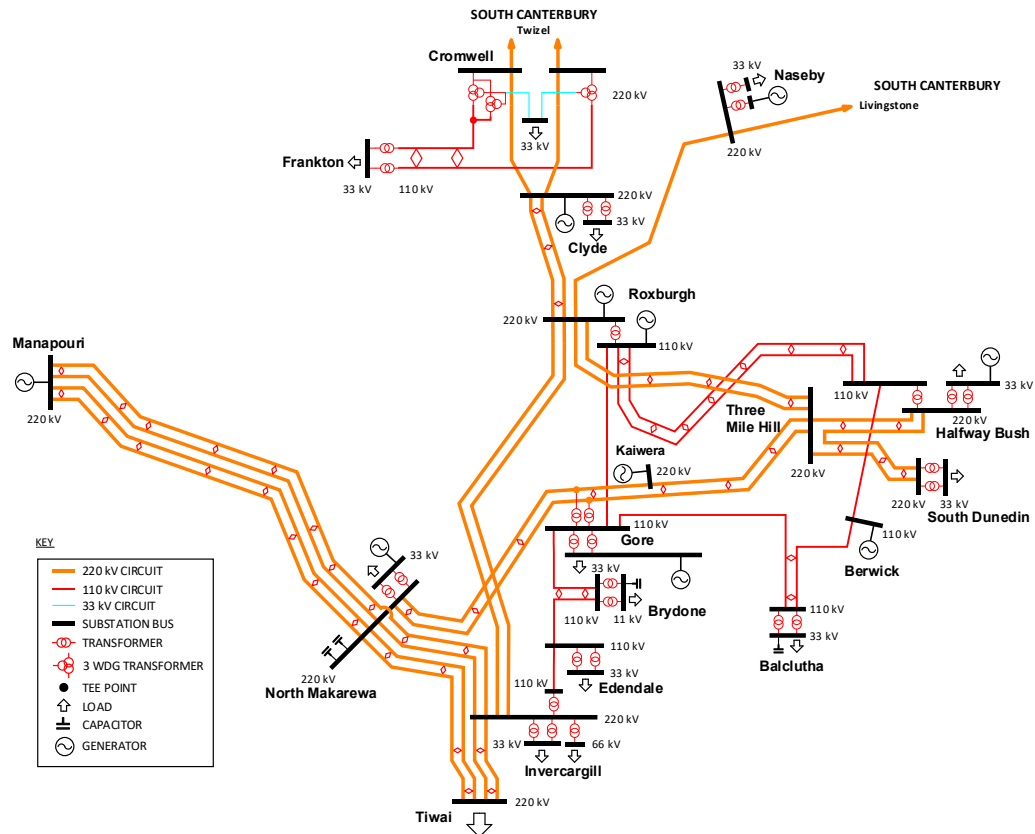
Figure 19-2: Otago-Southland region transmission schematic
