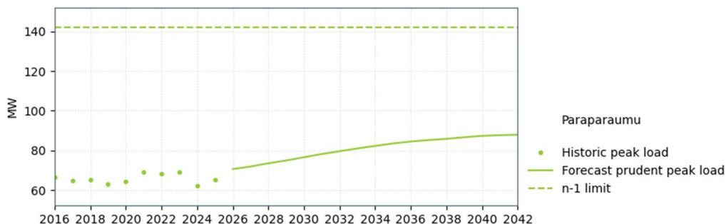
Figure 14-15: Paraparaumu supply capacity
