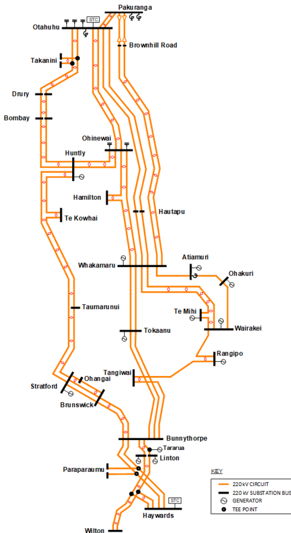
Figure 6-2: Simplified North Island grid backbone schematic
