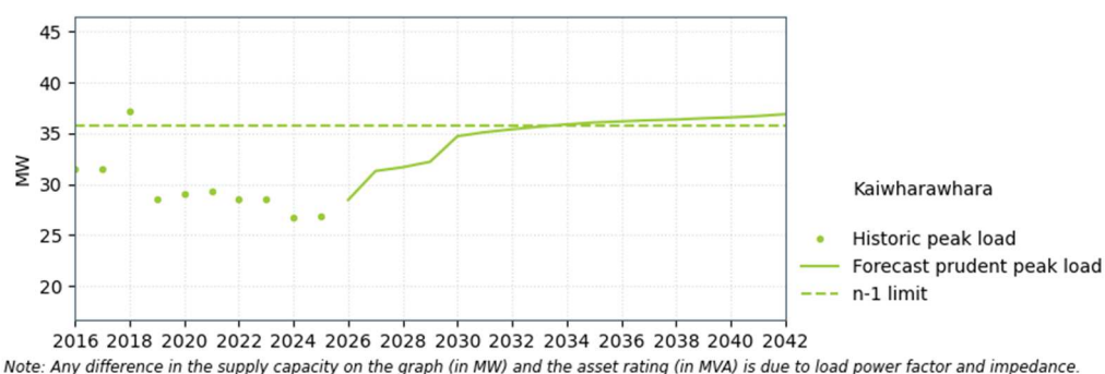
Figure 14-11: Kaiwharawhara supply capacity
