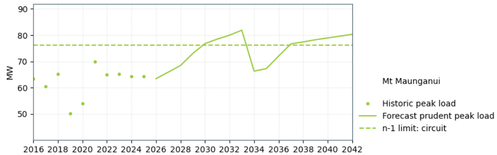
Figure 10-7: Mount Maunganui transmission capacity
