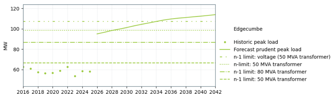
Figure 10-10: Edgecumbe supply capacity
