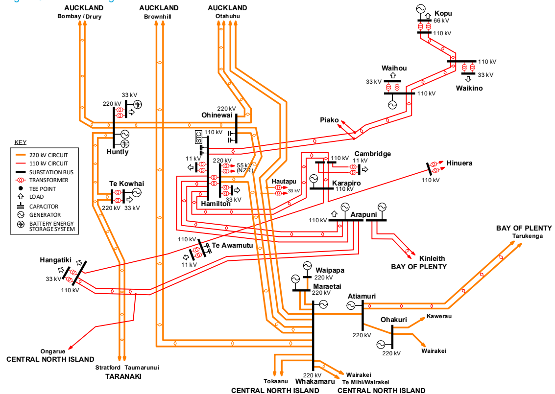
Figure 9-2: Waikato region transmission schematic
