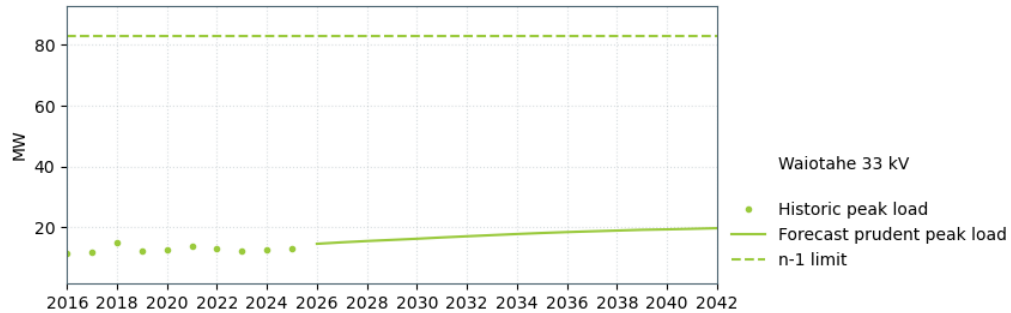
Figure 10-24: Waitoatahe supply capacity
