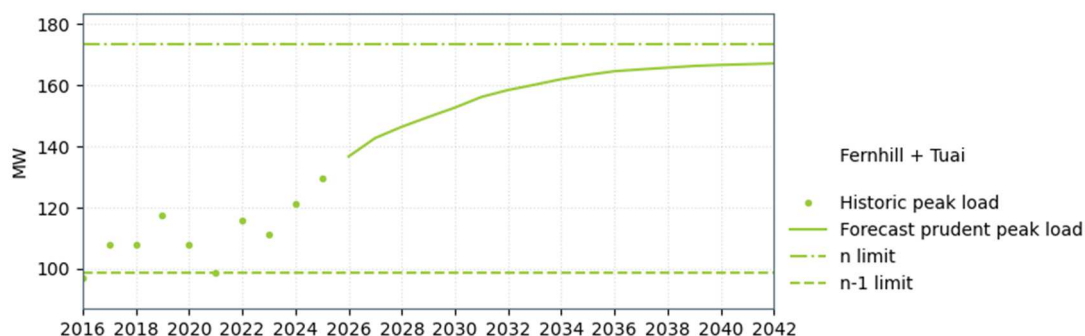
Figure 13-6: Fernhill–Redclyffe transmission capacity (with 25 MW Waikaremoana generation)
