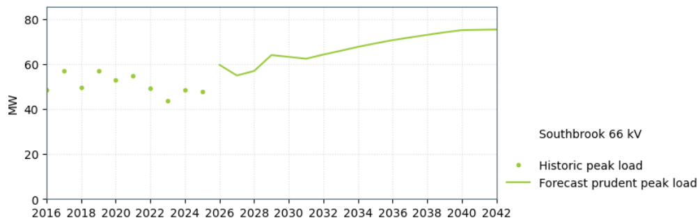
Figure 17-21: Southbrook 66 kV load forecast
