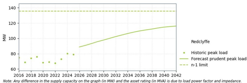
Figure 13-8: Redclyffe supply capacity
