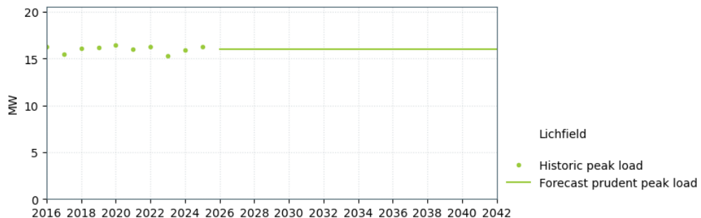
Figure 10-14: Lichfield load forecast
