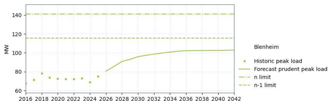
Figure 15-4: Blenheim supply capacity
