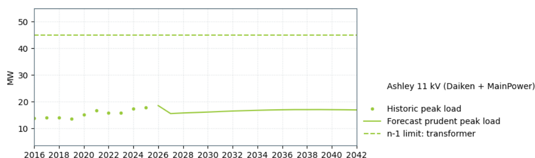
Figure 17-8: Ashley 11 kV supply capacity
