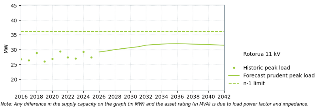
Figure 10-18: Rotorua 110/11 kV supply capacity
