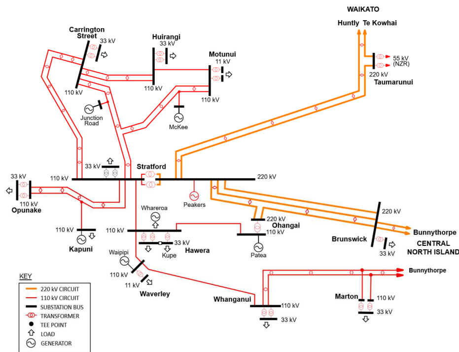
Figure 12-2: Taranaki region transmission schematic
