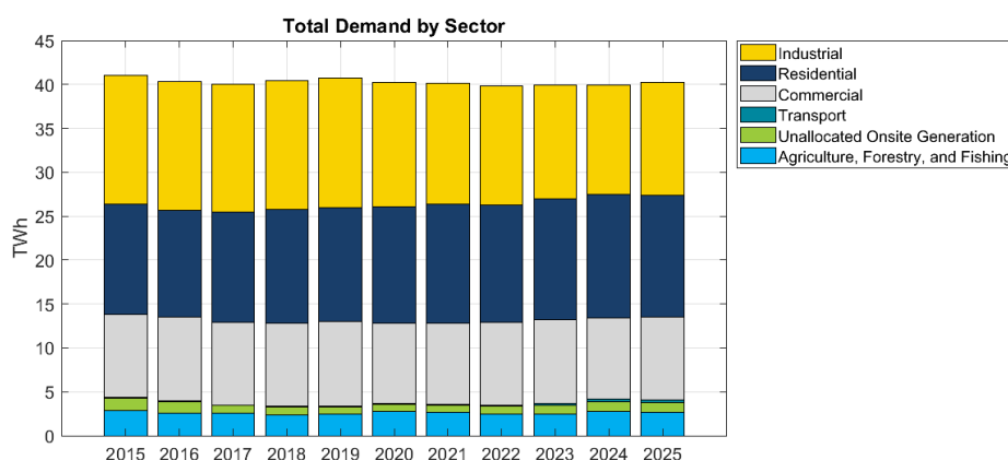
Figure 2-5: evolution of New Zealand gross electricity demand by sector (TWh)
