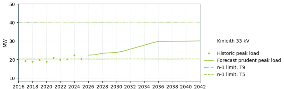
Figure 10-13: Kinleith 33 kV supply capacity
