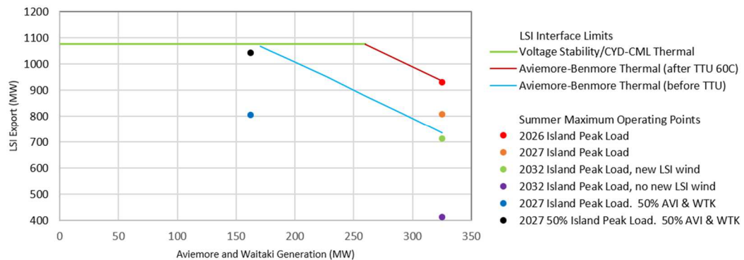
Figure 6-14: Lower South Island summer export limits
