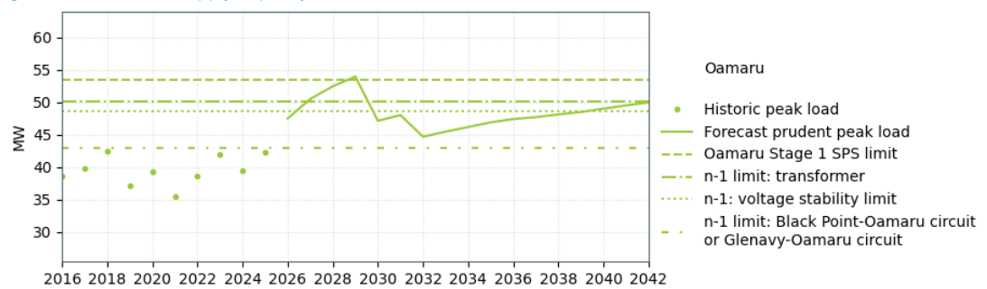
Figure 18-8: Oamaru supply capacity
