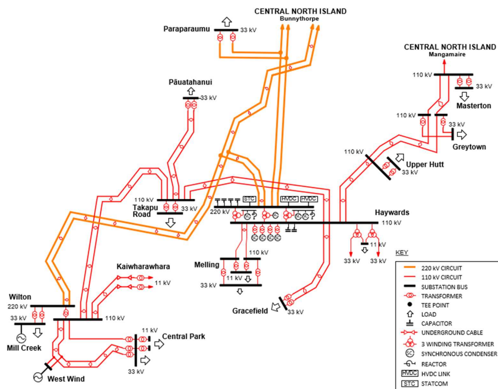
Figure 14-2: Wellington region transmission schematic
