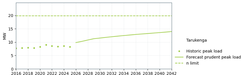
Figure 10-20: Tarukenga supply capacity
