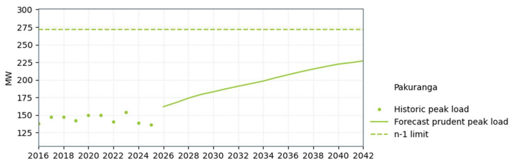
Figure 8-16: Pakuranga supply capacity
