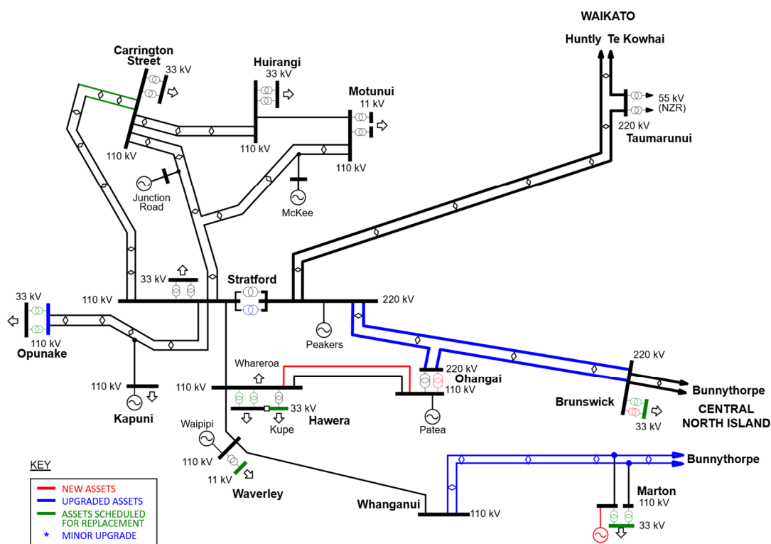
Figure 12-3: Possible Taranaki transmission configuration in 2041
