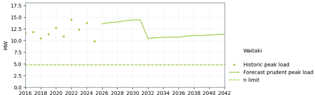
Figure 18-14: Waitaki load forecast and n limit provided by Transpower step-up transformer
