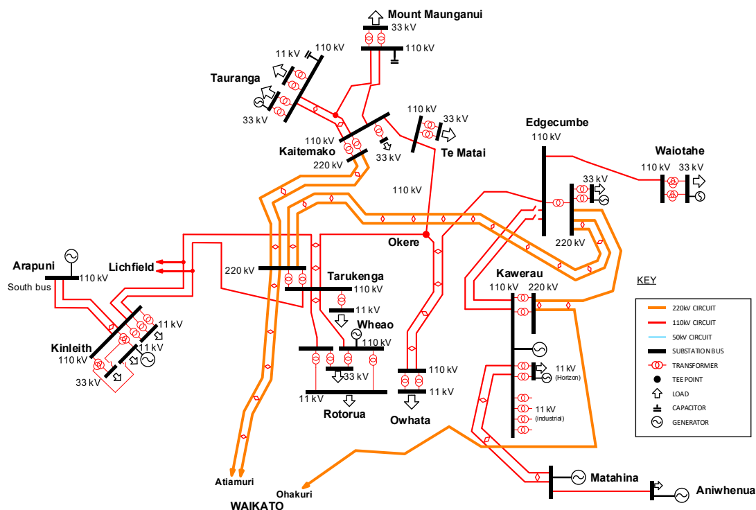
Figure 10-2: Bay of Plenty region transmission schematic
