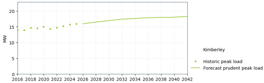
Figure 17-19: Kimberley load forecast
