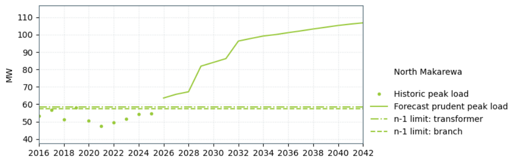
Figure 19-18: North Makarewa 33 kV supply capacity
