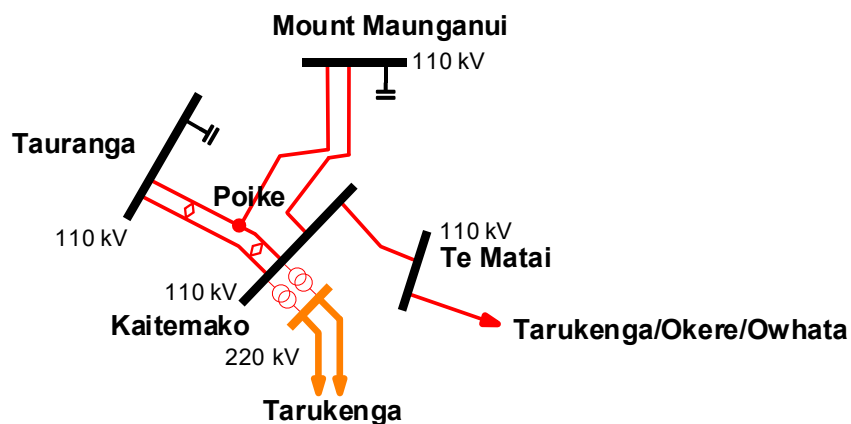
Figure 10-4: Kaitemako 220 kV and 110 kV grid configuration
