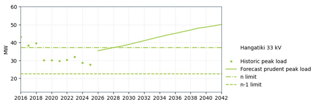
Figure 9-13: Hangatiki 33 kV supply capacity
