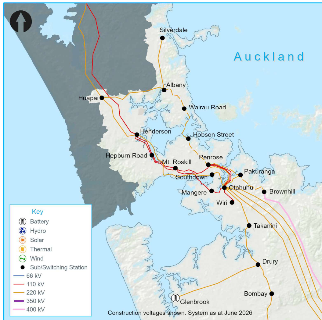
Figure 8-1: Auckland region transmission network map
