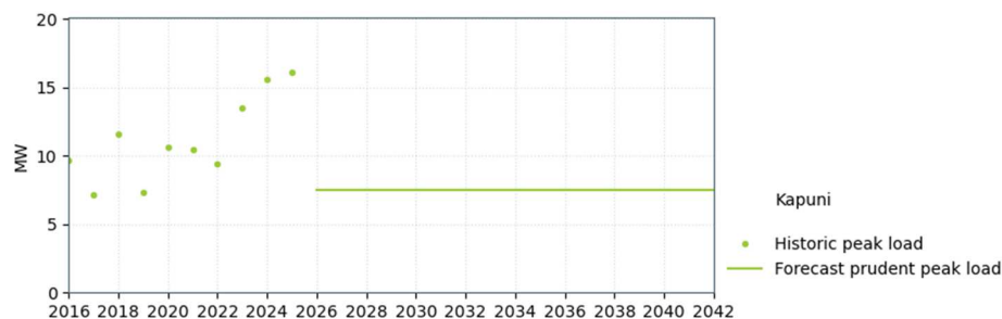
Figure 12-10: Kapuni load forecast
