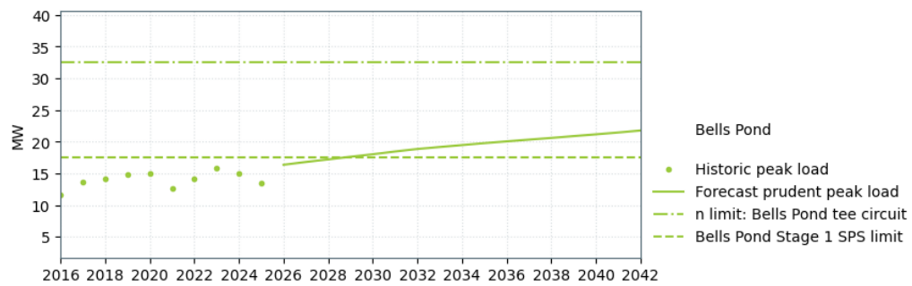
Figure 18-6: Bells Pond supply capacity
