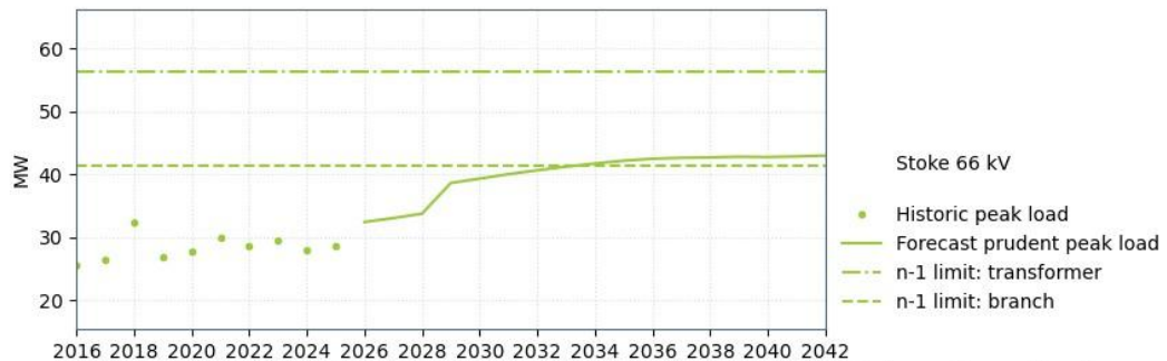
Figure 15-6: Stoke 66 kV supply capacity
