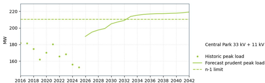
Figure 14-5: Central Park 110/33 kV supply capacity (combined 11 kV and 33 kV load)
