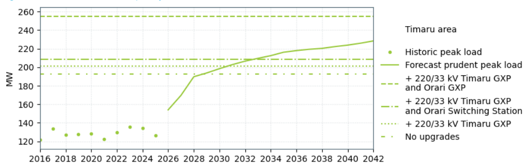
Figure 18-4: Timaru area capacity
