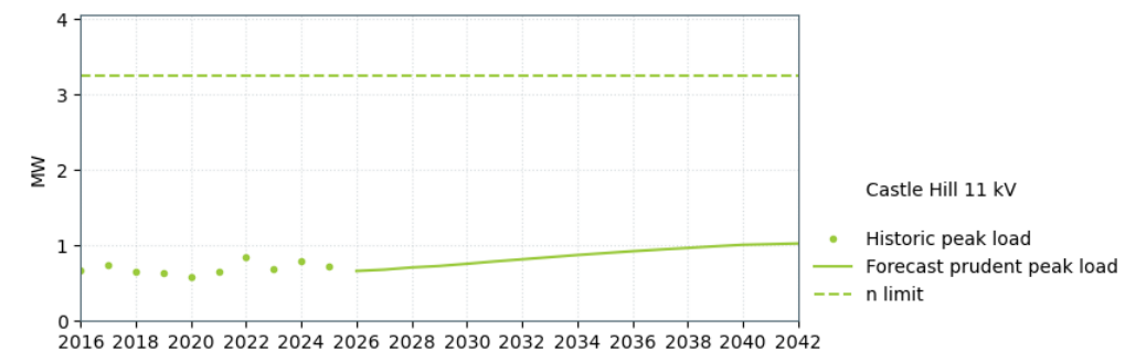
Figure 16-5: Castle Hill supply capacity
