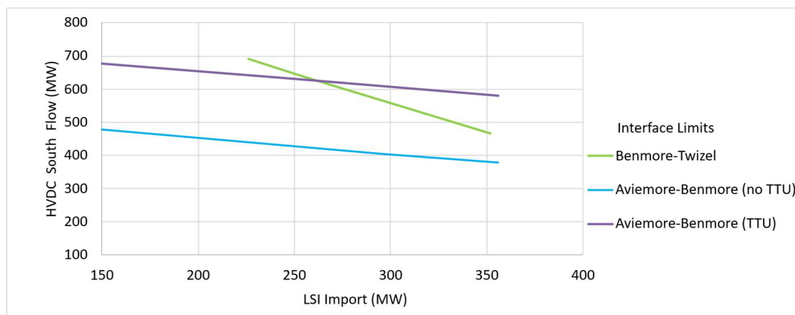
Figure 6-15: Waitaki Valley limits under high LSI import conditions
