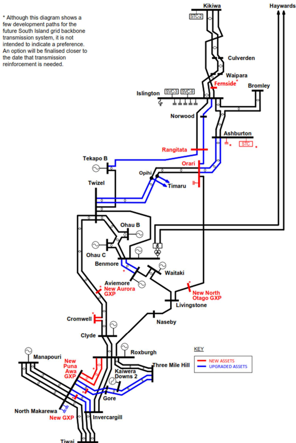
Figure 6-12: Possible South Island grid backbone schematic in 2041
