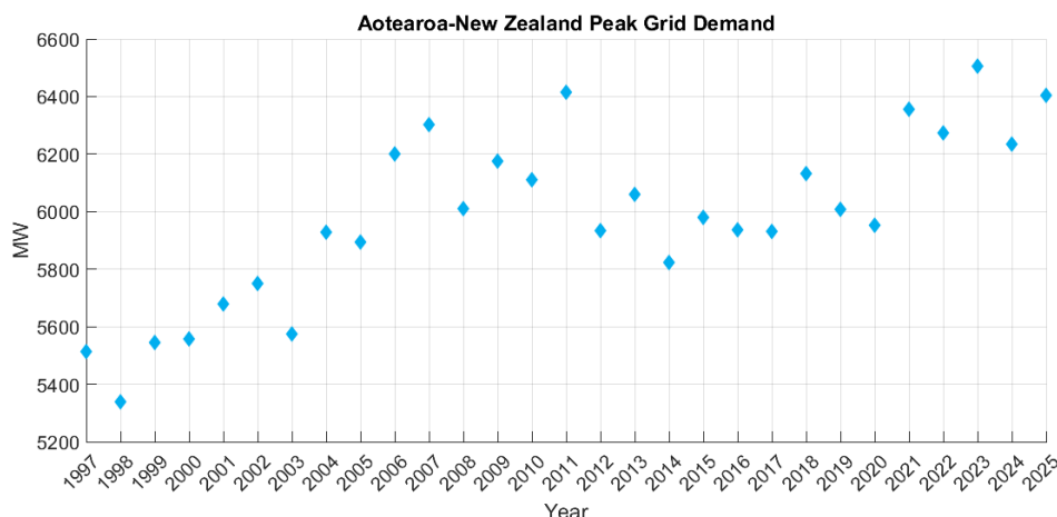
Figure 3-1: New Zealand peak grid demand (MW)
