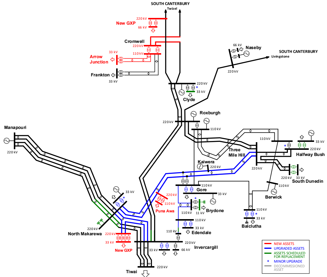
Figure 19-3: Possible Otago-Southland transmission configuration in 2041
