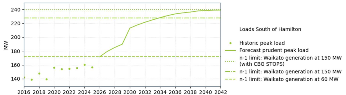
Figure 9-4: Cambridge–Hamilton circuit section capacity
