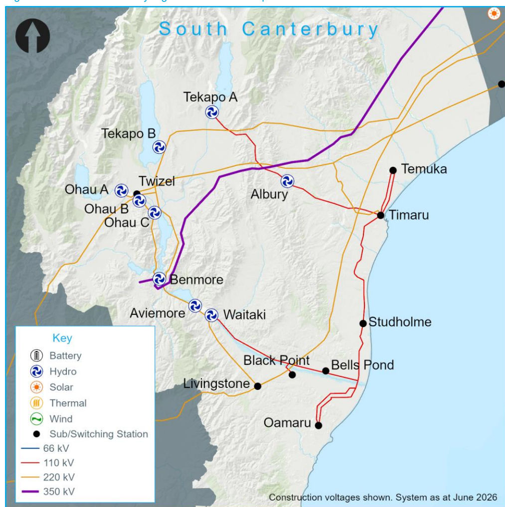
Figure 18-1: South Canterbury region transmission map
