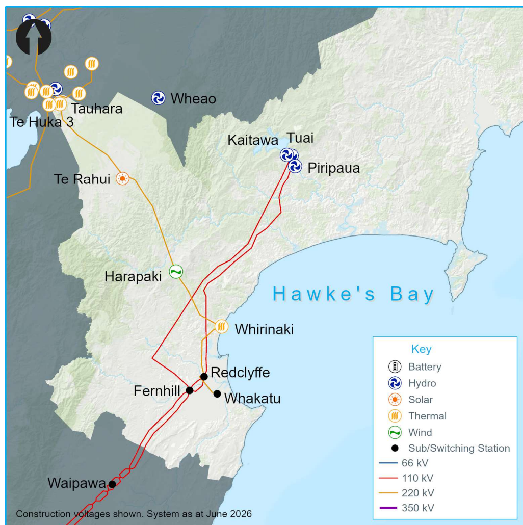
Figure 13-1: Hawke's Bay region transmission network map
