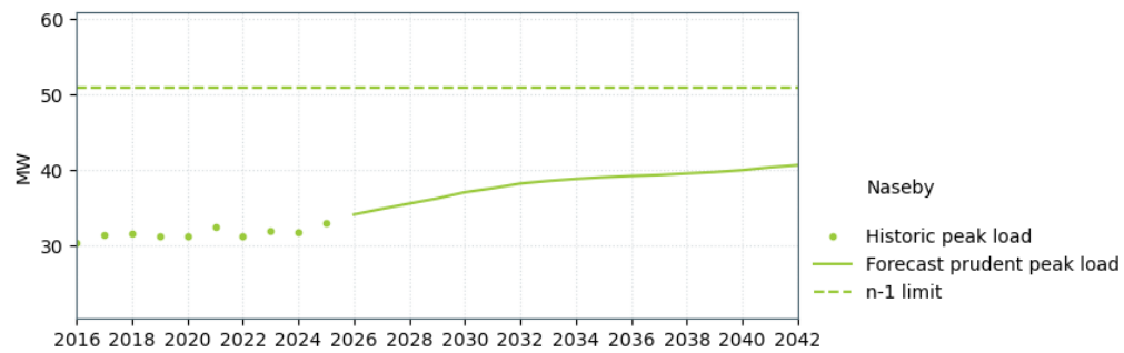
Figure 19-17: Naseby supply capacity
