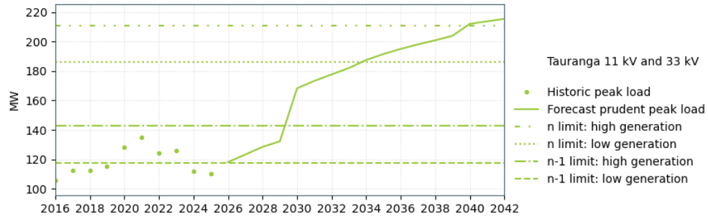
Figure 10-5: Kaitemako–Tauranga transmission capacity for low (14 MW), medium (33 MW), and high (40 MW) Kaimai generation levels
