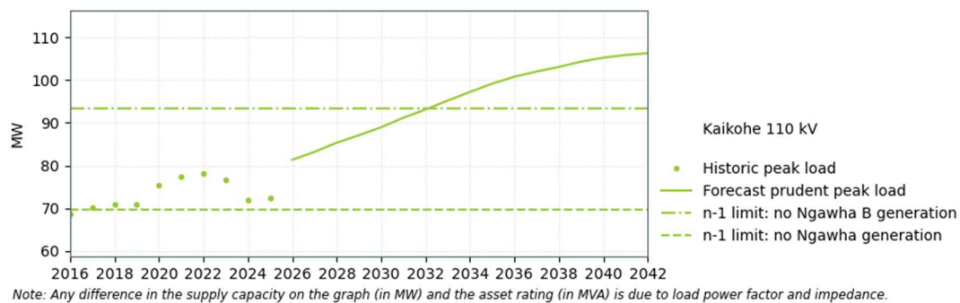
Figure 7-5: Kaikohe supply capacity
