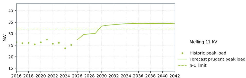
Figure 14-14: Melling 110/11 kV supply capacity
