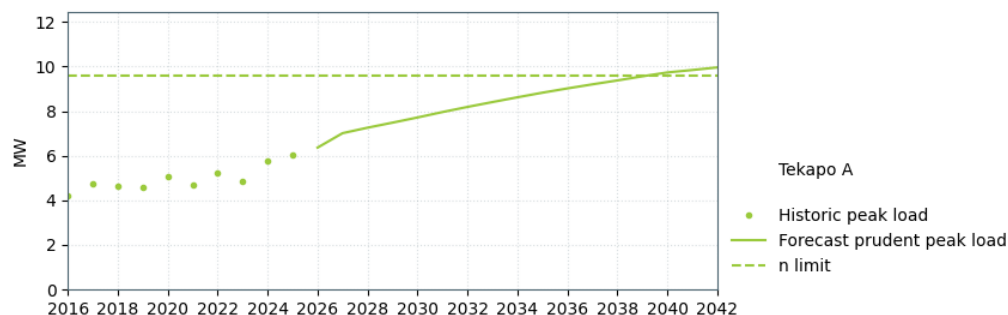
Figure 18-10: Tekapo A supply capacity
