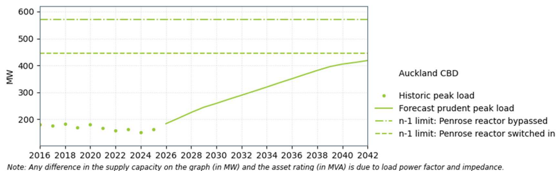
Figure 8-4: Auckland CBD supply capacity
