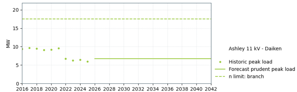
Figure 17-7: Ashley 11 kV supply capacity – Daiken
