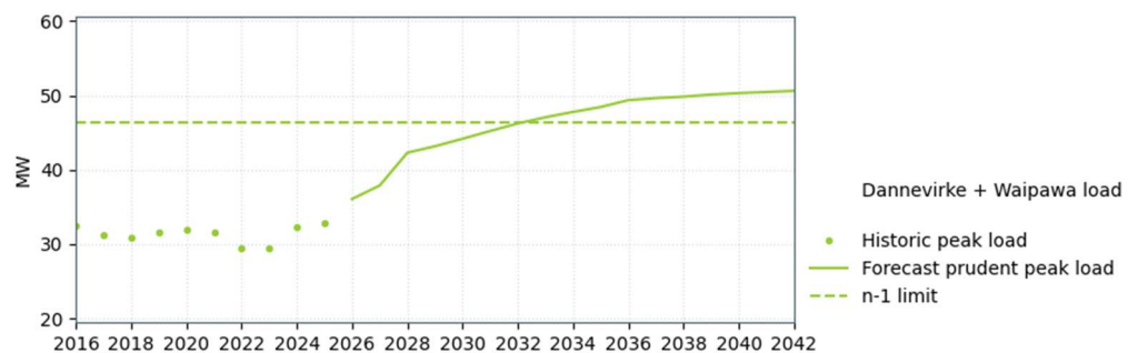
Figure 11-4: Dannevirke–Woodville 110 kV circuit capacity
