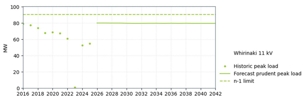
Figure 13-12: Whirinaki supply capacity
