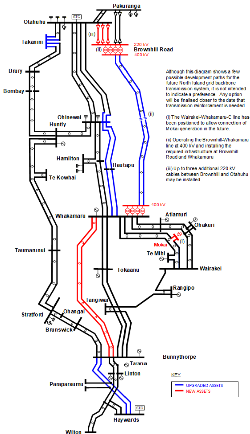
Figure 6-4: Longer-term indicative North Island grid backbone schematic (beyond 2041)
