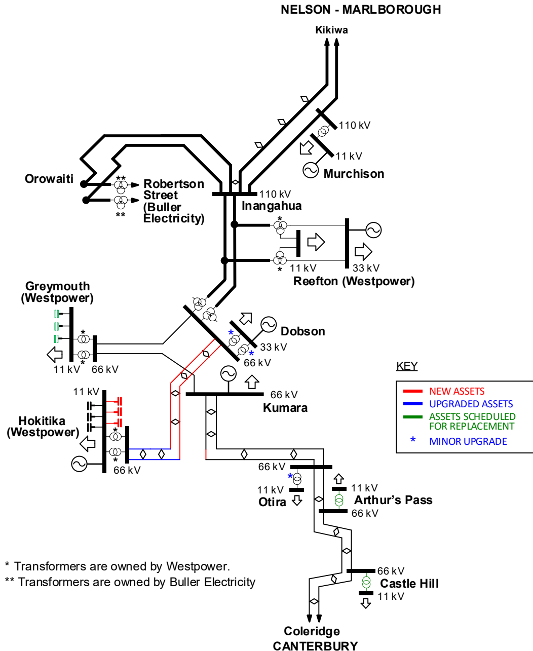
Figure 16-3: Possible West Coast transmission configuration in 2041
