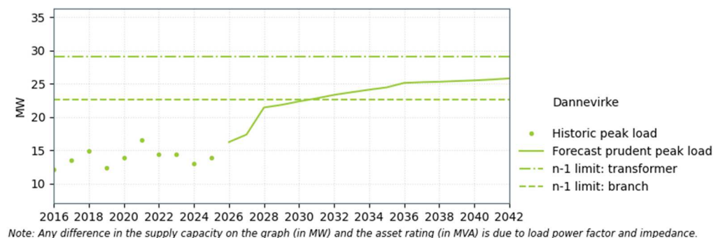
Figure 11-6: Dannevirke supply capacity
