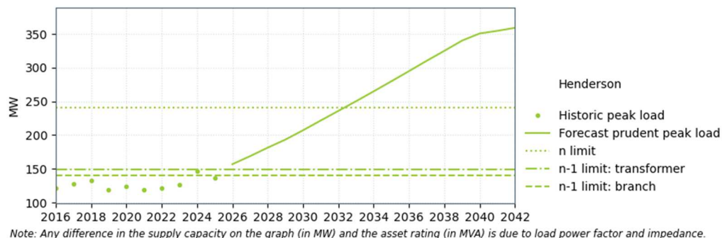
Figure 8-9: Henderson supply capacity
