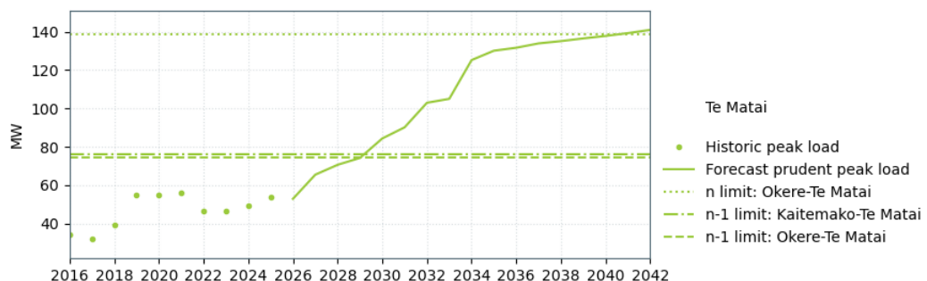
Figure 10-8: Te Matai transmission capacity
