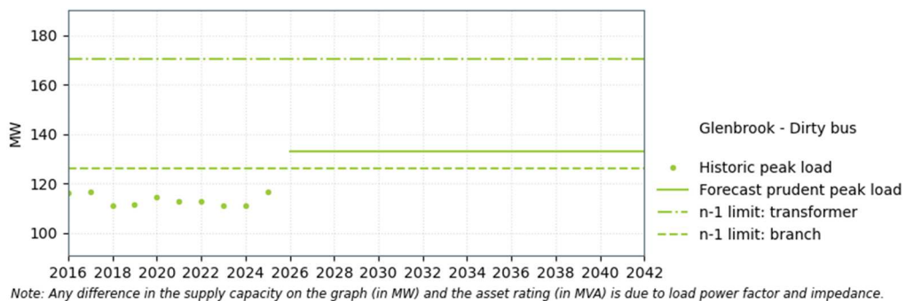
Figure 8-7: Glenbrook dirty bus supply capacity
