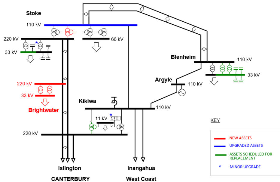
Figure 15-3: Possible Nelson-Marlborough transmission configuration in 2041
