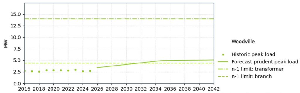
Figure 11-17: Woodville supply capacity
