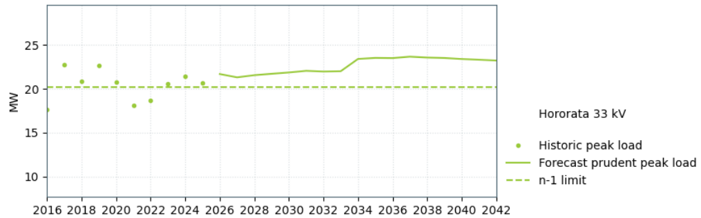
Figure 17-14: Hororata 33 kV supply capacity
