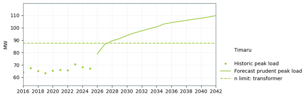
Figure 18-12: Timaru supply capacity
