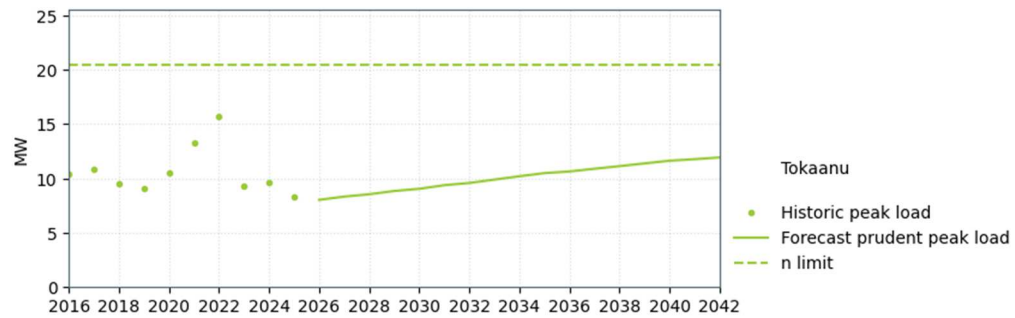
Figure 11-14: Tokaanu supply capacity
