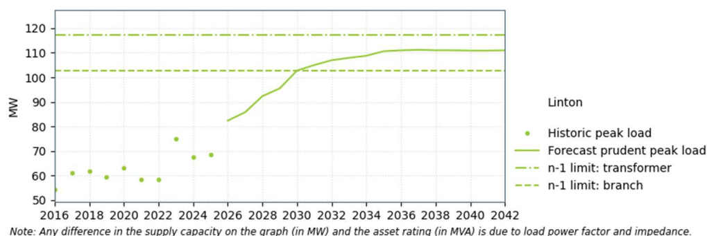
Figure 11-7: Linton supply capacity
