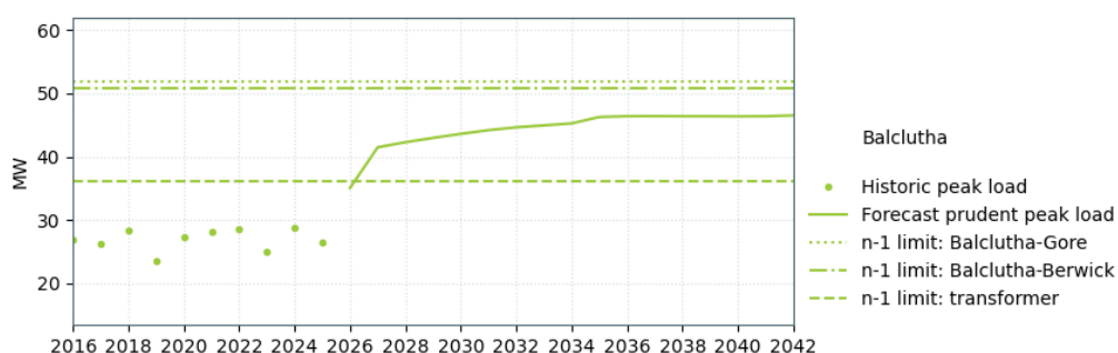
Figure 19-6: Balclutha supply capacity
