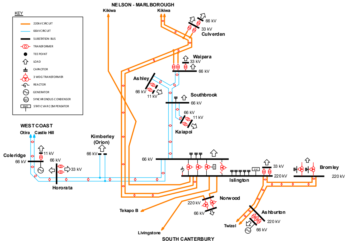
Figure 17-2: Canterbury region transmission schematic
