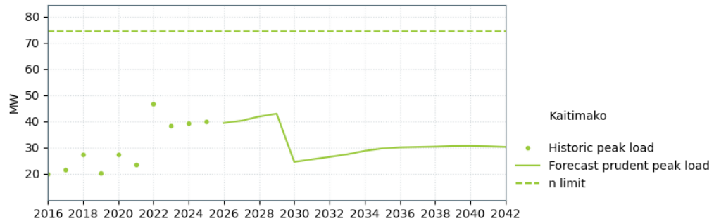
Figure 10-11: Kaitemako supply capacity
