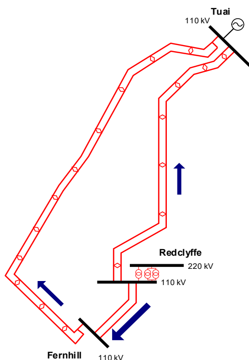
Figure 13-5: Power flow from Redclyffe to Tuai during high load and low generation at Tuai (with 25 MW Waikaremoana generation)
