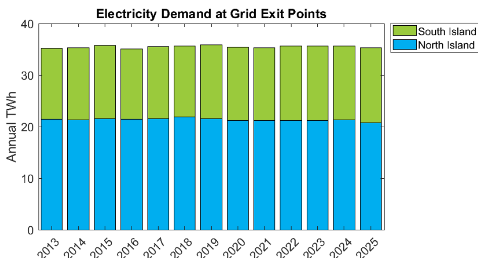
Figure 2-4: New Zealand grid exit point electricity demand (TWh)
