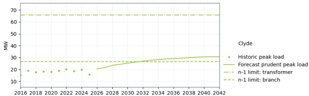
Figure 19-8: Clyde supply capacity
