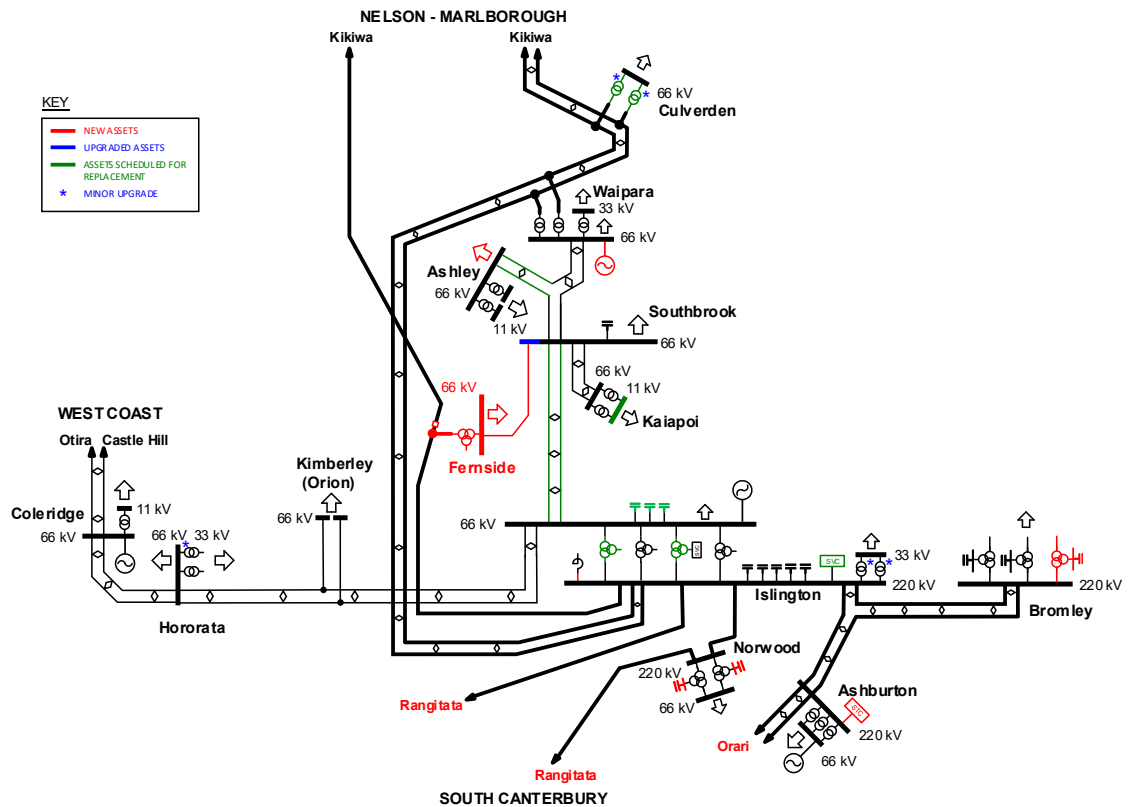
Figure 17-3: Possible Canterbury transmission configuration in 2041
