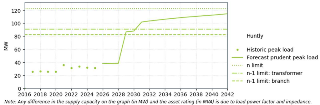
Figure 9-16: Huntly supply capacity
