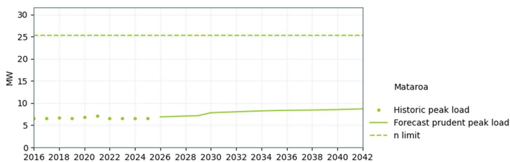
Figure 11-10: Mataroa supply capacity
