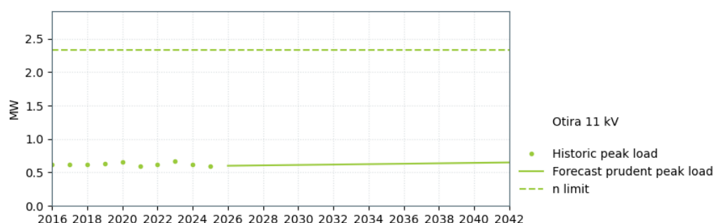
Figure 16-11: Otira supply capacity
