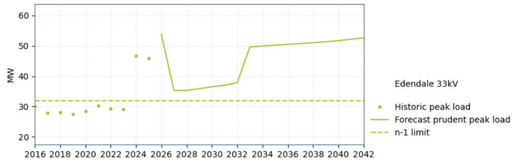
Figure 19-10: Edendale 33 kV supply capacity
