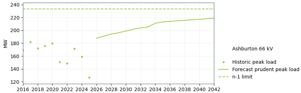
Figure 17-5: Ashburton supply capacity
