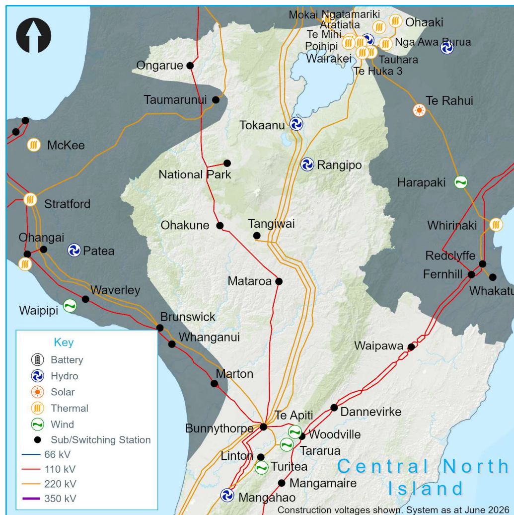
Figure 11-1: Central North Island region transmission map
