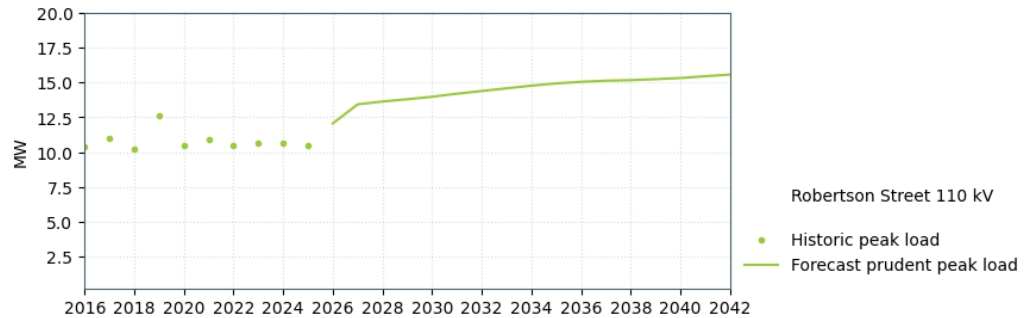
Figure 16-13: Robertson Street load forecast
