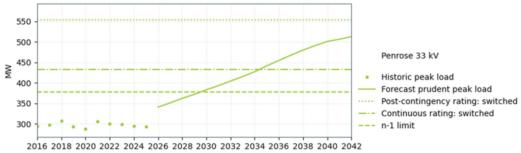
Figure 8-18: Penrose 33 kV supply capacity
