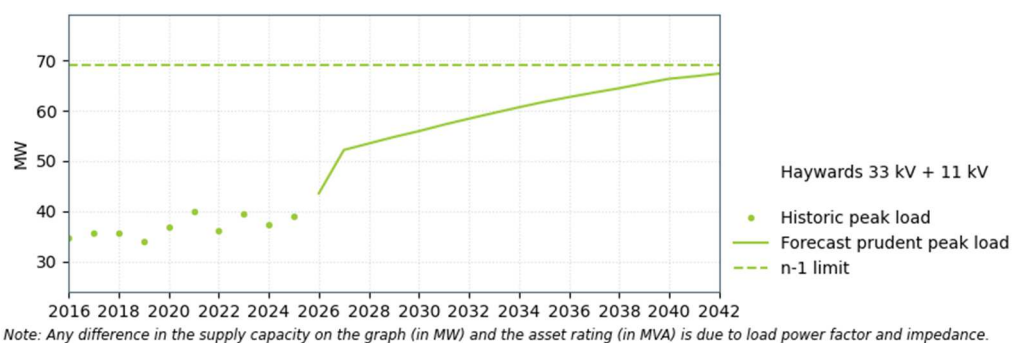
Figure 14-10: Haywards supply capacity (combined 33 kV and 11 kV load)
