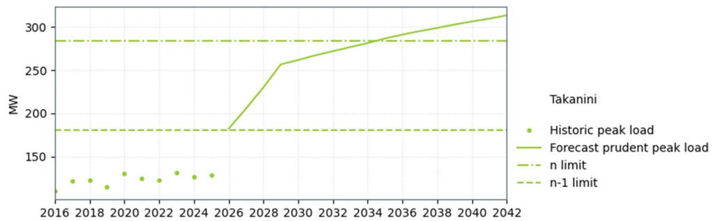
Figure 8-20: Takanini supply capacity
