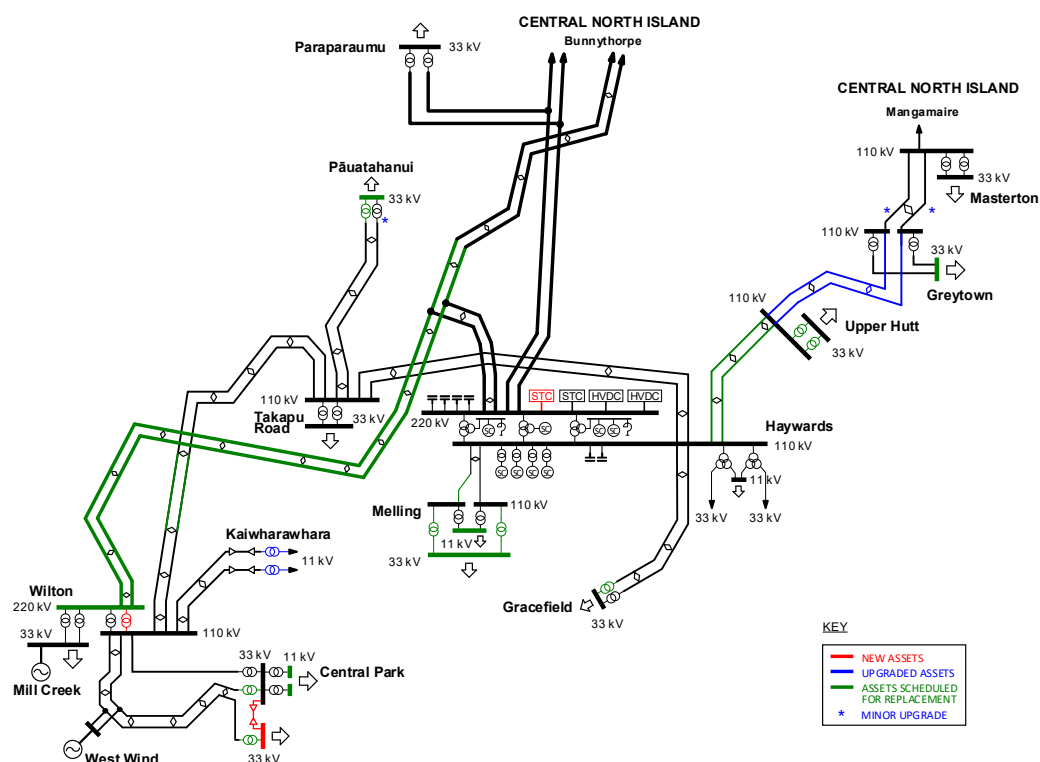
Figure 14-3: Possible Wellington transmission configuration in 2041
