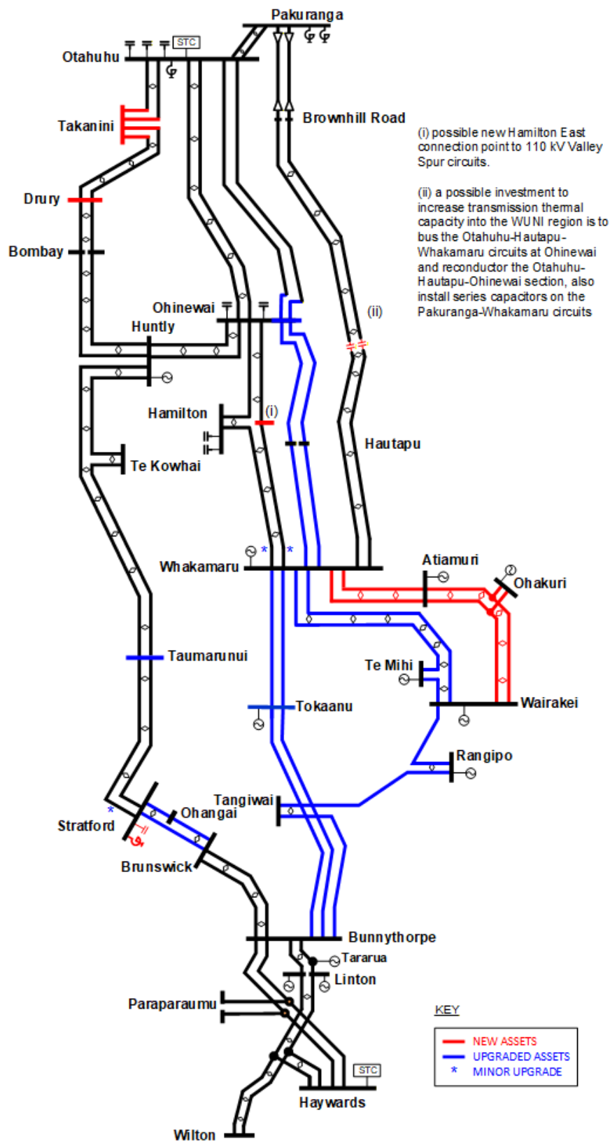
Figure 6-3: Indicative North Island grid backbone schematic to 2041
