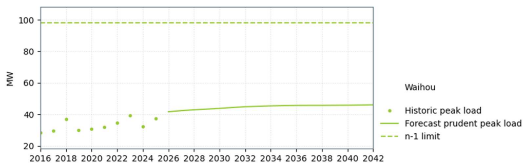
Figure 9-22: Waihou supply capacity
