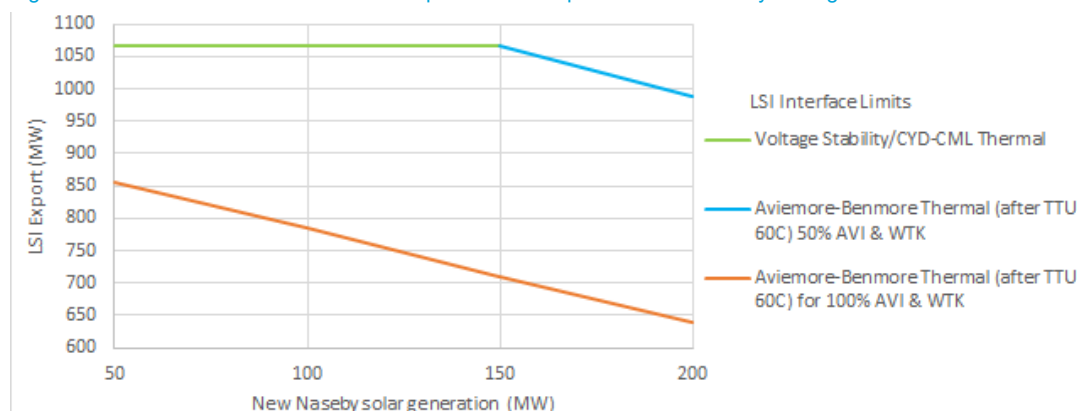
Figure 6-16: Lower South Island summer export limits with possible new Naseby solar generation
