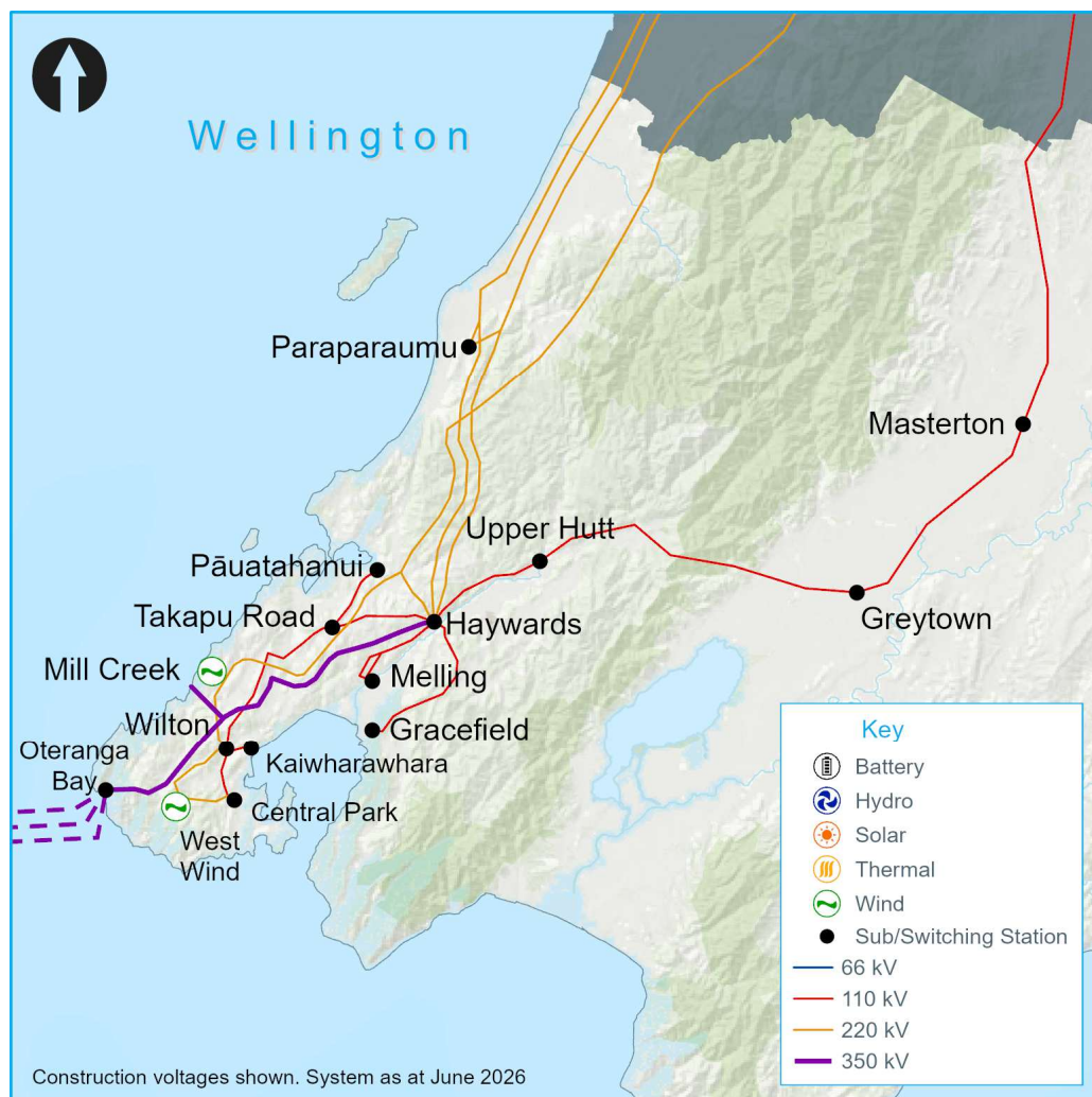
Figure 14-1: Wellington region transmission network map
