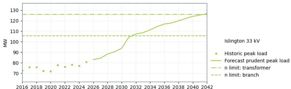
Figure 17-16: Islington 33 kV supply capacity
