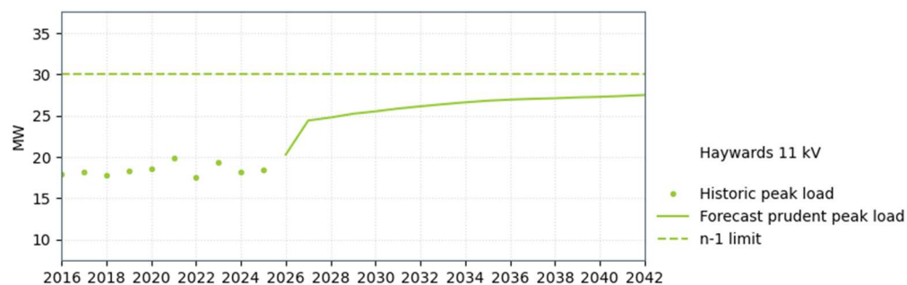
Figure 14-9: Haywards 11 kV and 33 kV supply capacity
