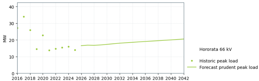
Figure 17-15: Hororata 66 kV load forecast
