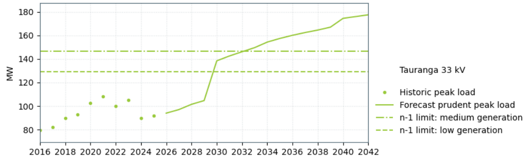
Figure 10-21: Tauranga 110/33 kV supply capacity for low (14 MW) and medium (33 MW) Kaimai generation
