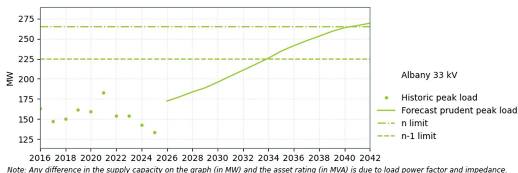
Figure 8-5: Albany supply capacity
