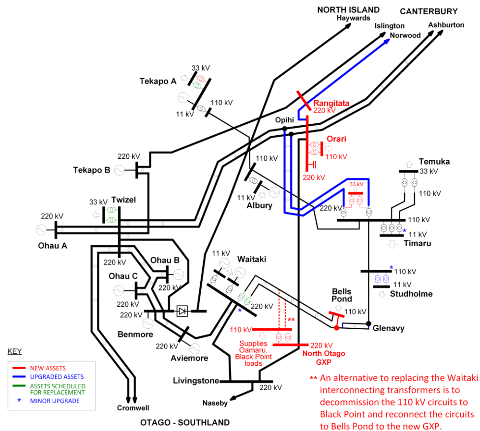
Figure 18-3: Possible South Canterbury transmission configuration in 2041
