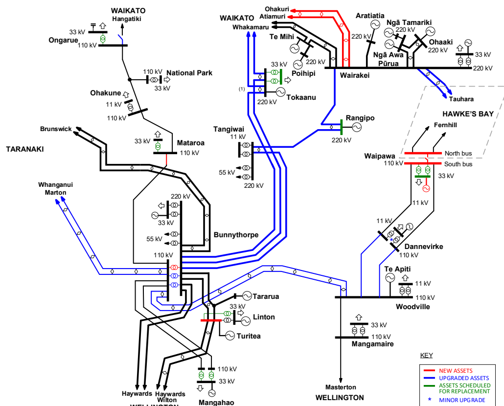
Figure 11-3: Possible Central North Island transmission configuration in 2041
