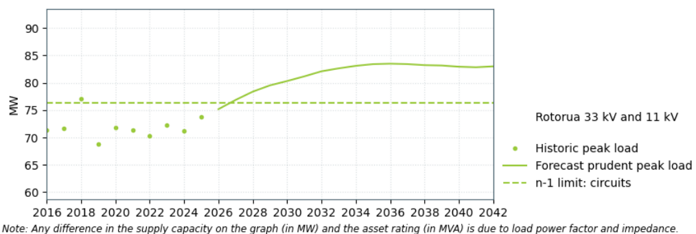
Figure 10-19: Rotorua–Tarukenga transmission capacity
