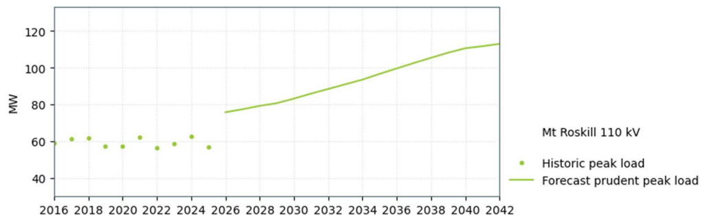
Figure 8-13: Mount Roskill 110 kV load forecast
