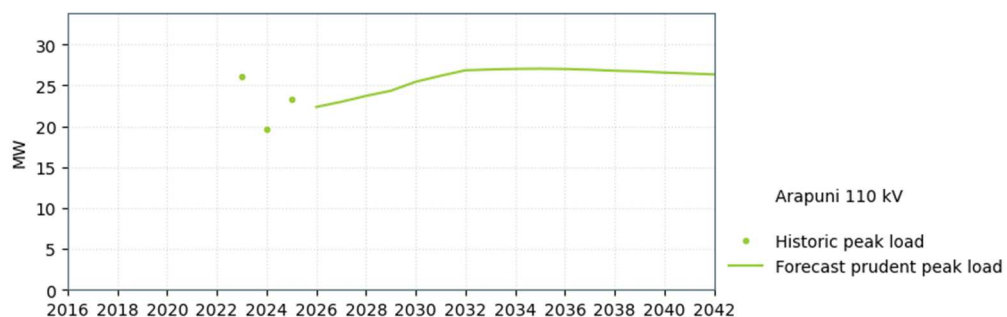
Figure 9-8: Arapuni load forecast
