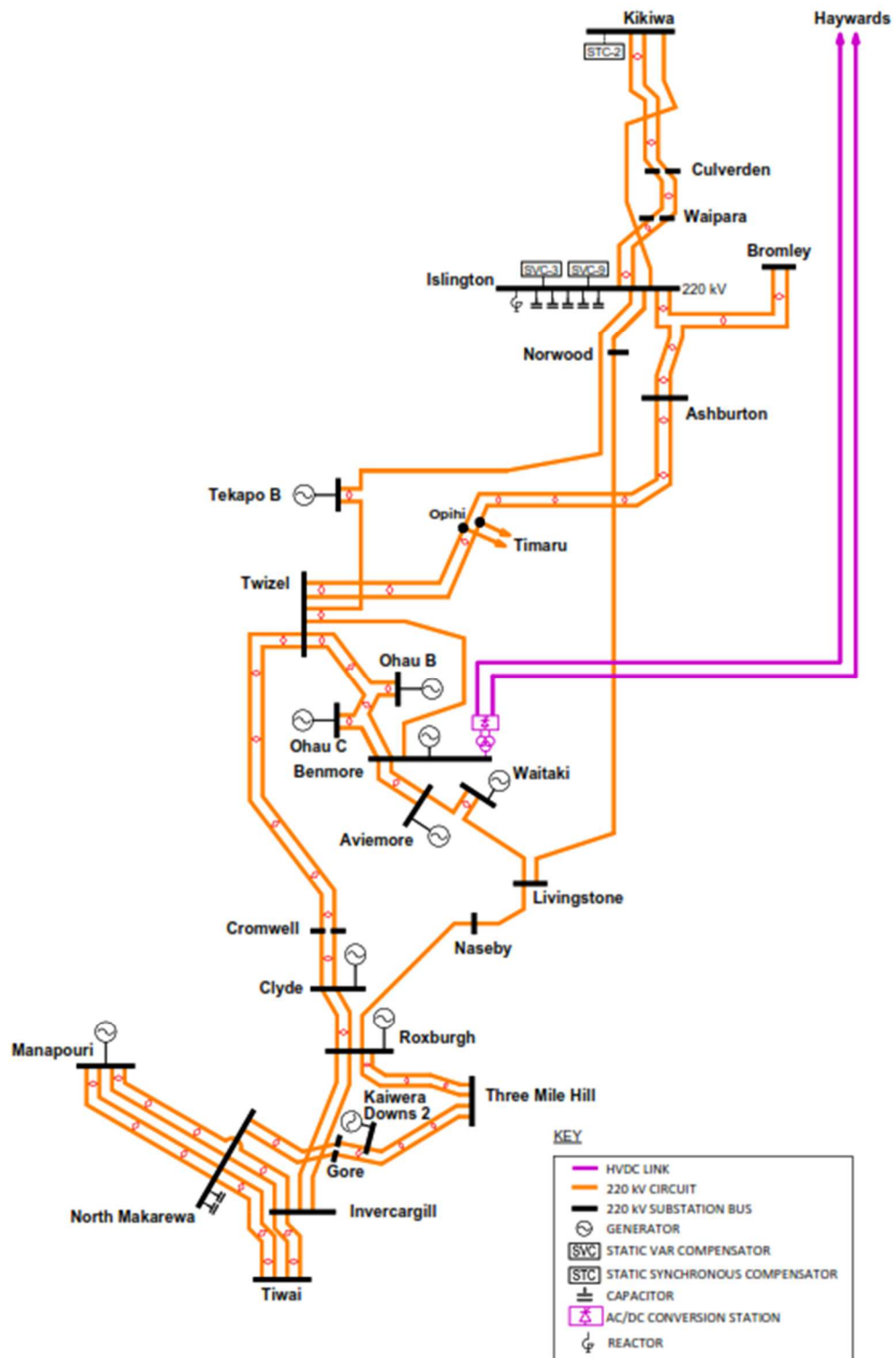
Figure 6-11: South Island grid backbone schematic
