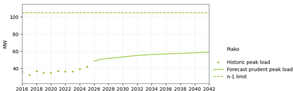
Figure 9-18: Piako supply capacity (Piako–Morrinsville Tee n-1 capacity)
