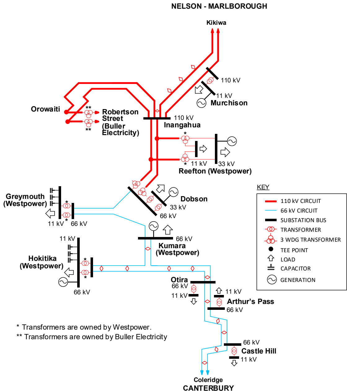
Figure 16-2: West Coast transmission schematic
