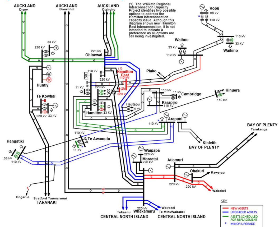
Figure 9-3: Possible Waikato transmission configuration in 2041
