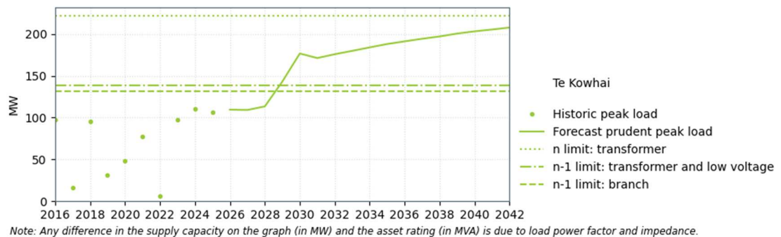
Figure 9-20: Te Kowhai supply capacity and low voltage with no contribution from Te Uku
