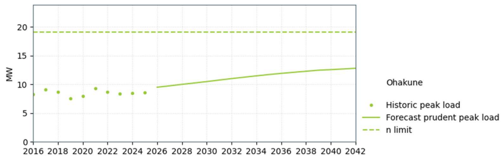
Figure 11-12: Ohakune supply capacity
