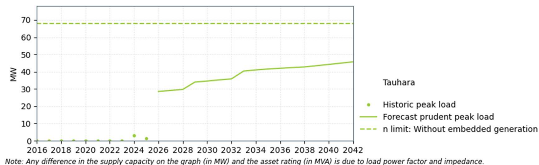
Figure 13-9: Tauhara supply capacity
