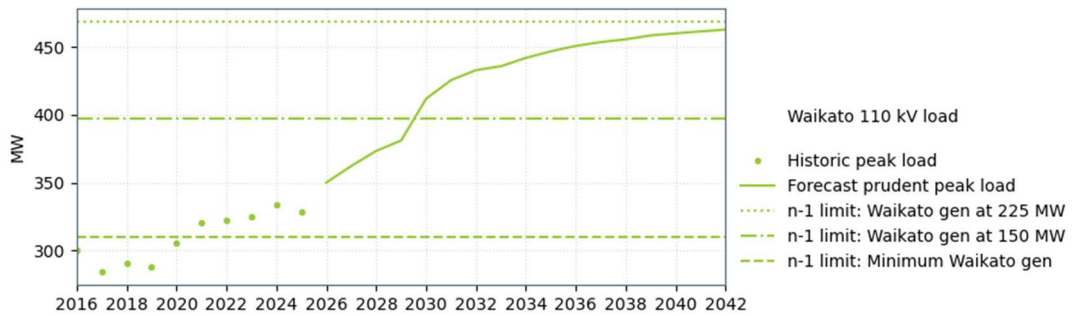
Figure 9-7: Waikato 110 kV supply capacity
