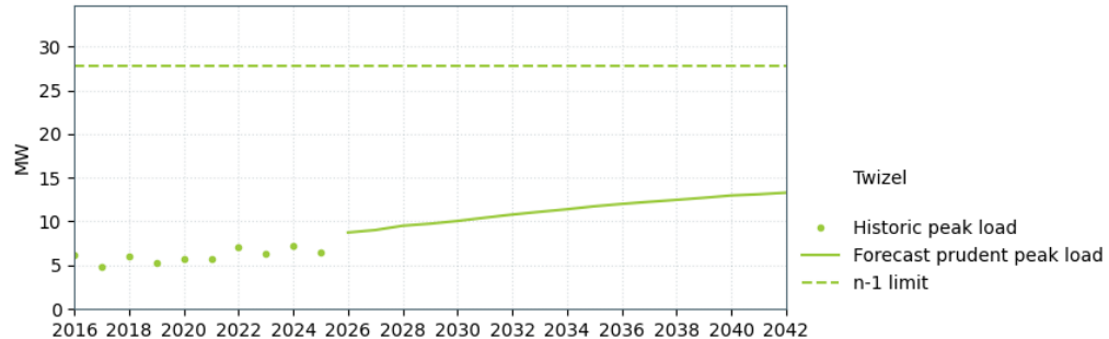
Figure 18-13: Twizel supply capacity
