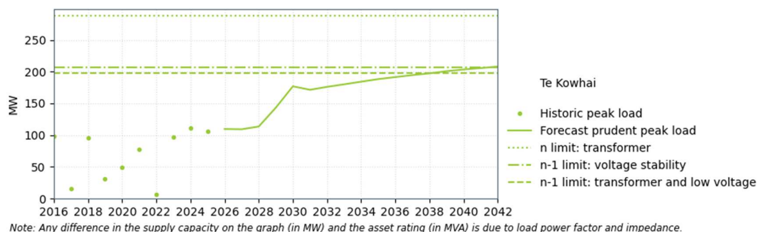
Figure 9-21: Te Kowhai supply capacity and low voltage with 67 MW contribution from Te Uku generation
