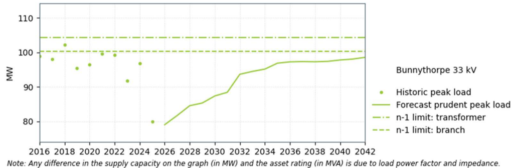
Figure 11-5: Bunnythorpe supply capacity
