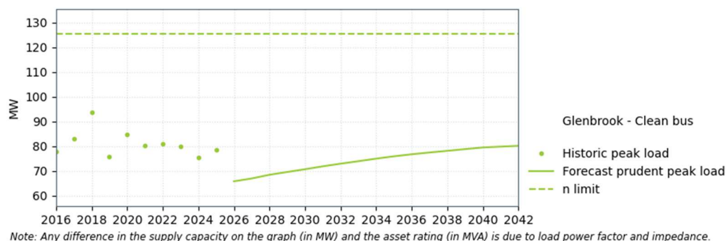
Figure 8-8: Glenbrook clean bus supply capacity without cogeneration and BESS
