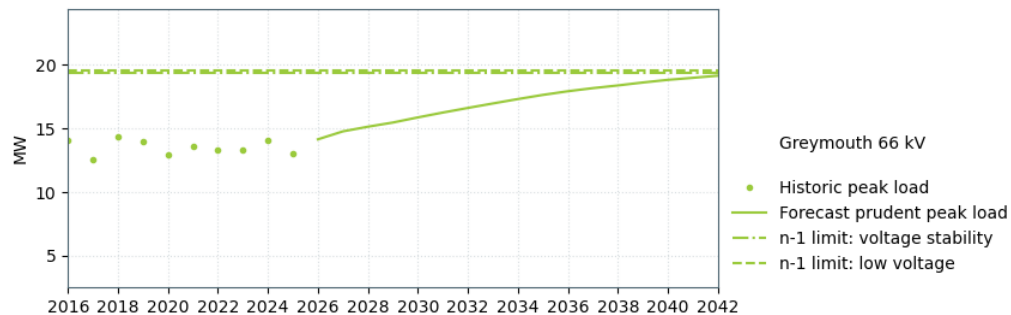
Figure 16-7: Greymouth transmission capacity
