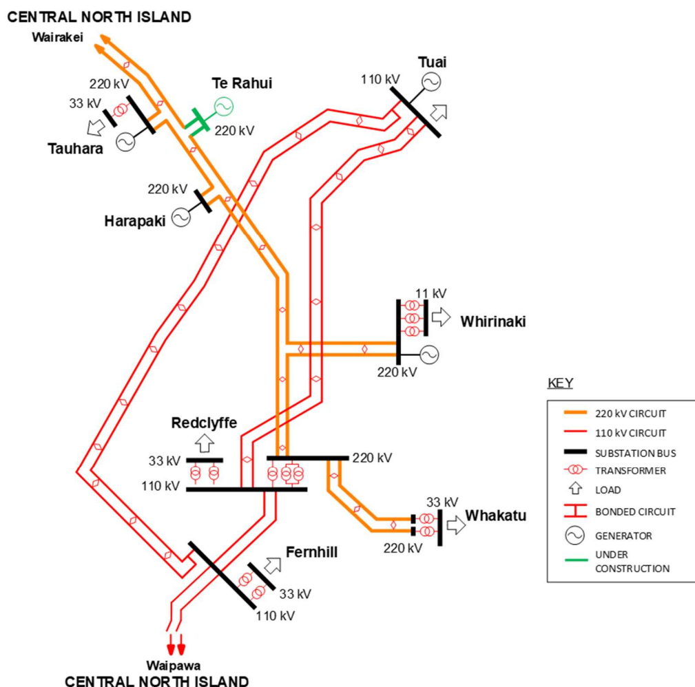
Figure 13-2: Hawke's Bay region transmission schematic
