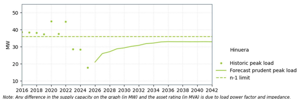
Figure 9-15: Hinuera supply capacity
