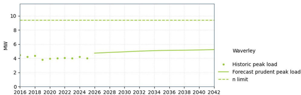
Figure 12-15: Waverley supply capacity
