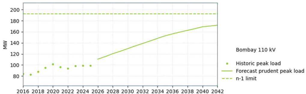
Figure 8-6: Bombay 110 kV supply capacity
