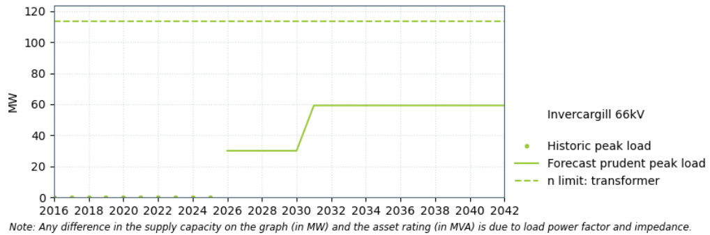
Figure 19-16: Invercargill 66 kV supply capacity
