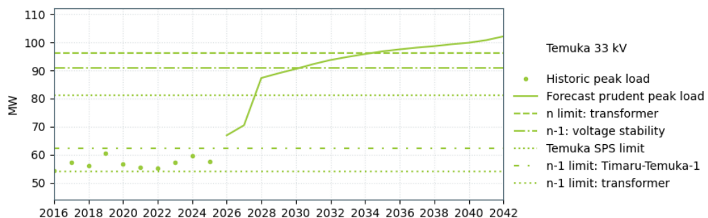
Figure 18-11: Temuka supply capacity: supply transformer
