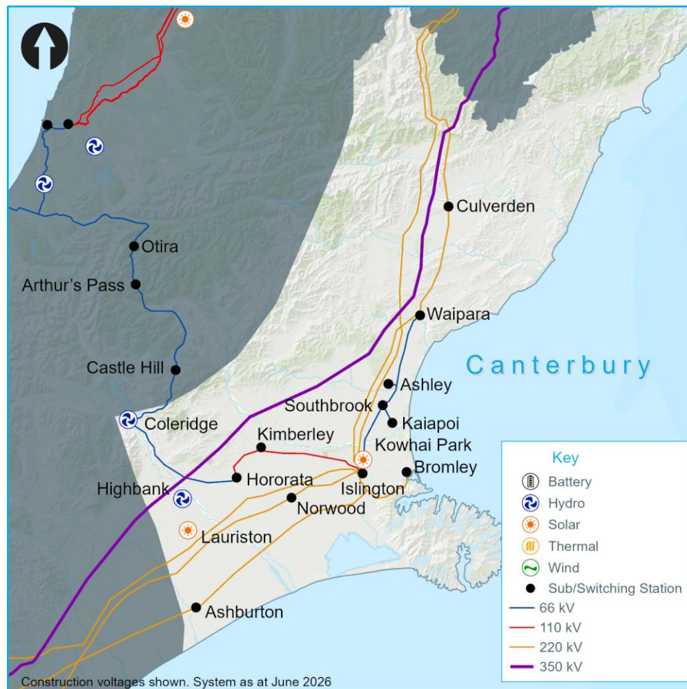
Figure 17-1: Canterbury region transmission network map
