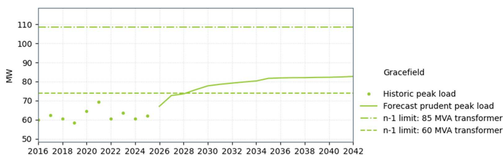
Figure 14-7: Gracefield supply capacity
