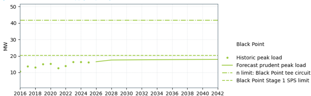
Figure 18-7: Black Point supply capacity
