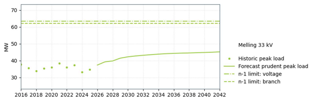
Figure 14-13: Melling 110/33 kV supply capacity
