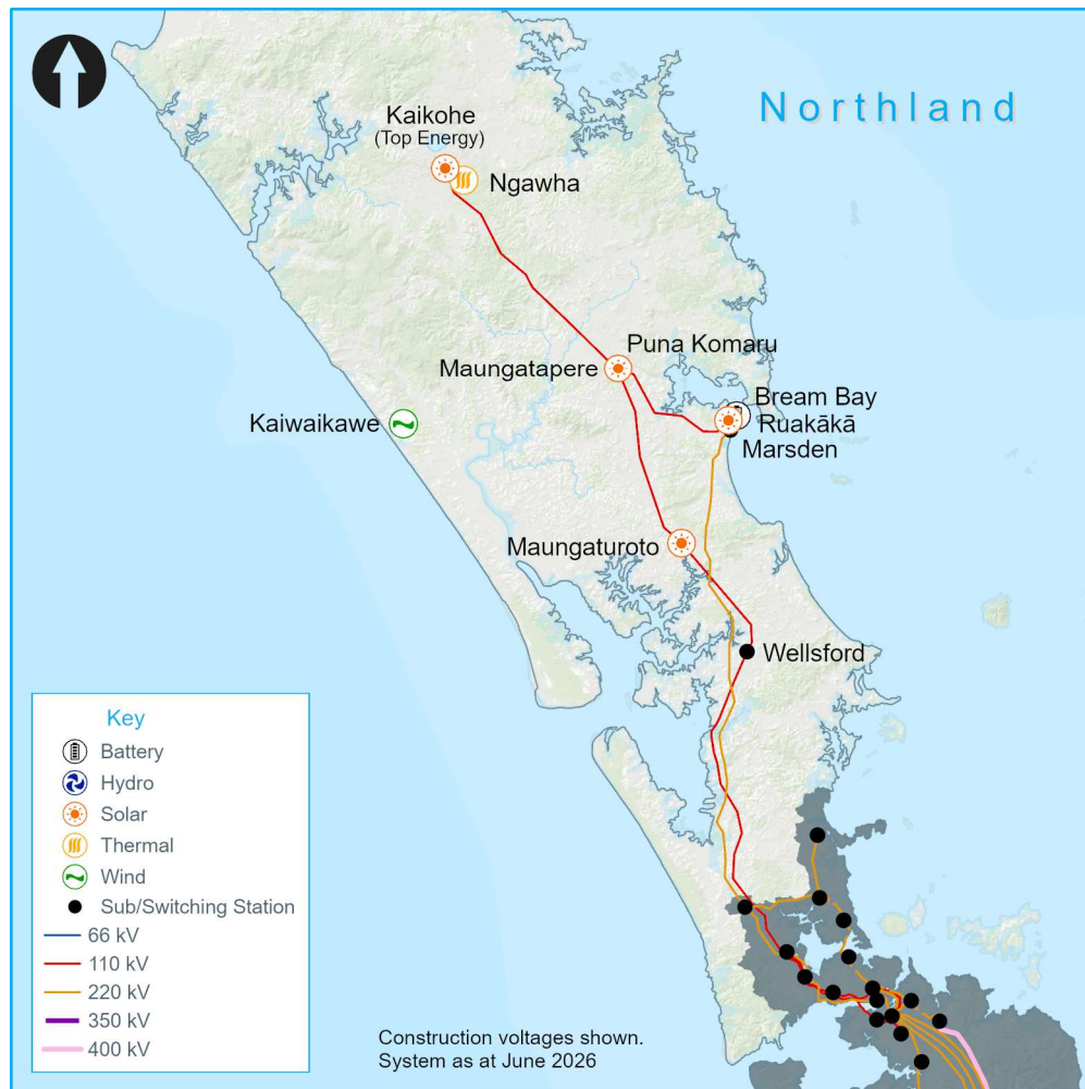
Figure 7-1: Northland region transmission network map
