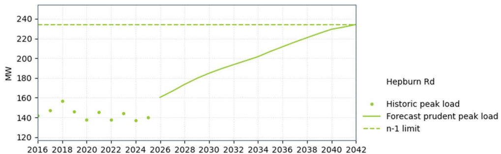
Figure 8-10: Hepburn Road supply capacity
