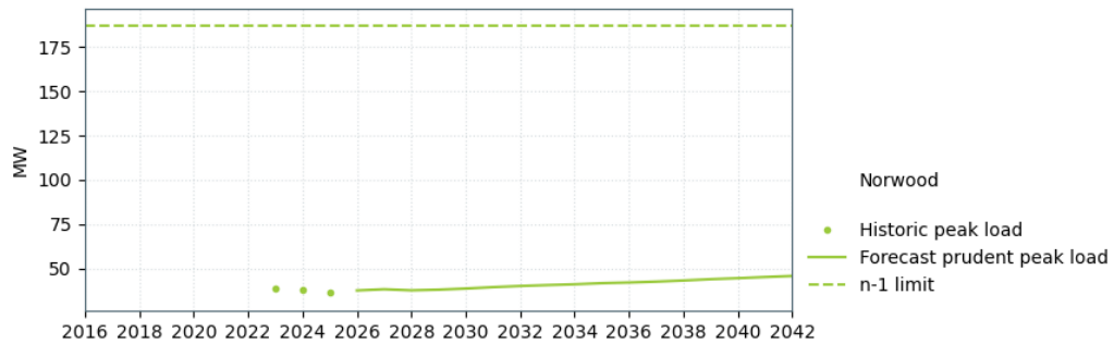
Figure 17-20: Norwood load forecast
