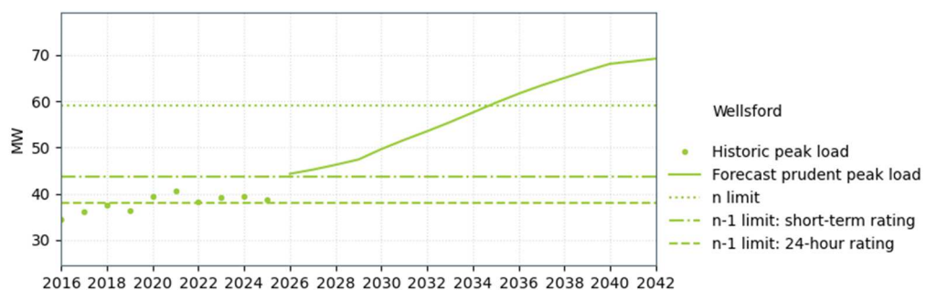
Figure 7-8: Wellsford supply capacity
