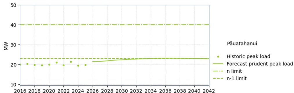
Figure 14-16: Pāuatahanui supply capacity
