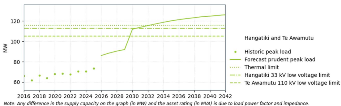
Figure 9-6: Hangatiki and Te Awamutu winter transmission capacity
