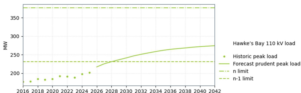
Figure 13-4: Redclyffe interconnecting transformer capacity (with 25 MW Waikaremoana generation)
