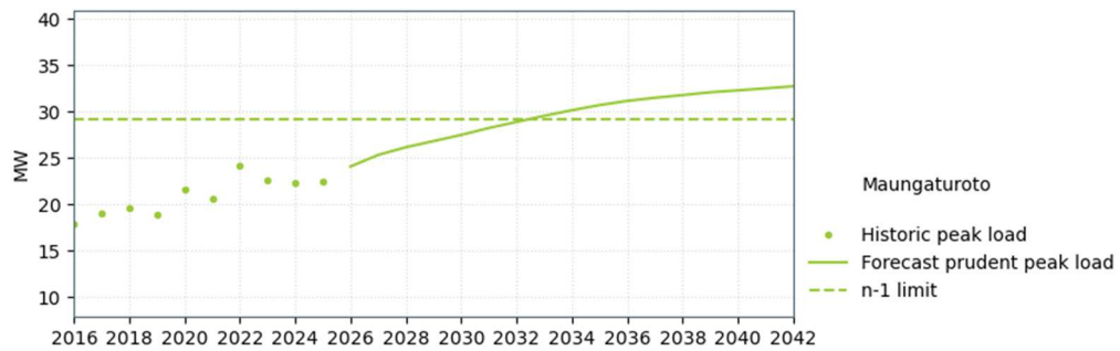
Figure 7-7: Maungaturoto supply capacity
