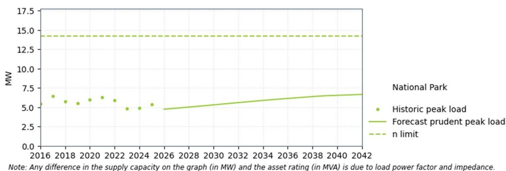
Figure 11-11: National Park supply capacity
