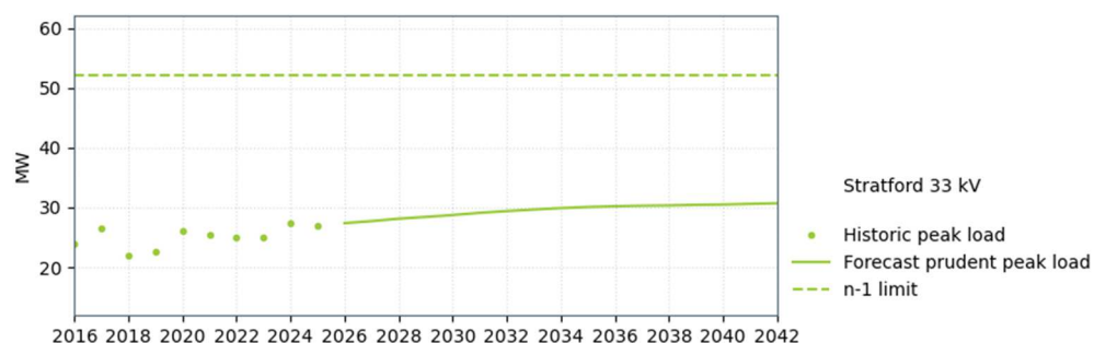
Figure 12-14: Stratford supply capacity
