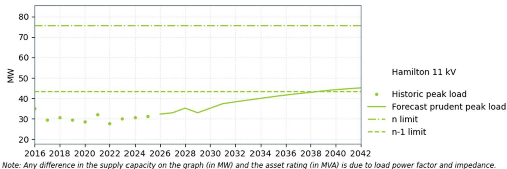
Figure 9-11: Hamilton 11 kV supply capacity
