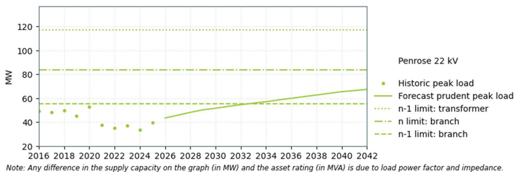
Figure 8-17: Penrose 22 kV supply capacity
