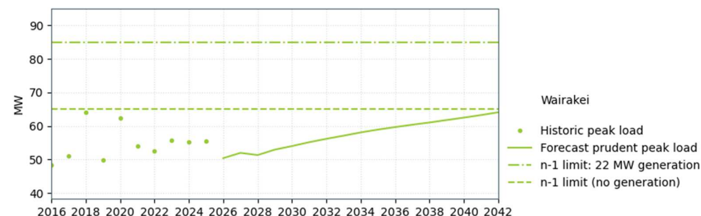
Figure 11-16: Wairakei supply capacity
