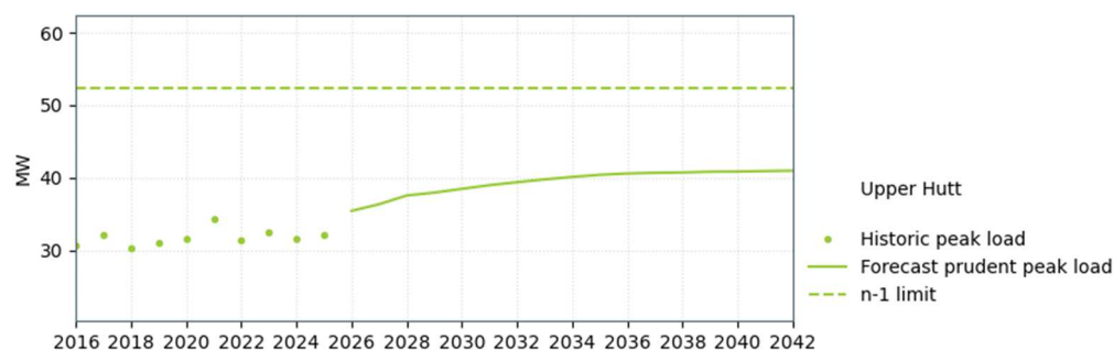
Figure 14-18: Upper Hutt supply capacity
