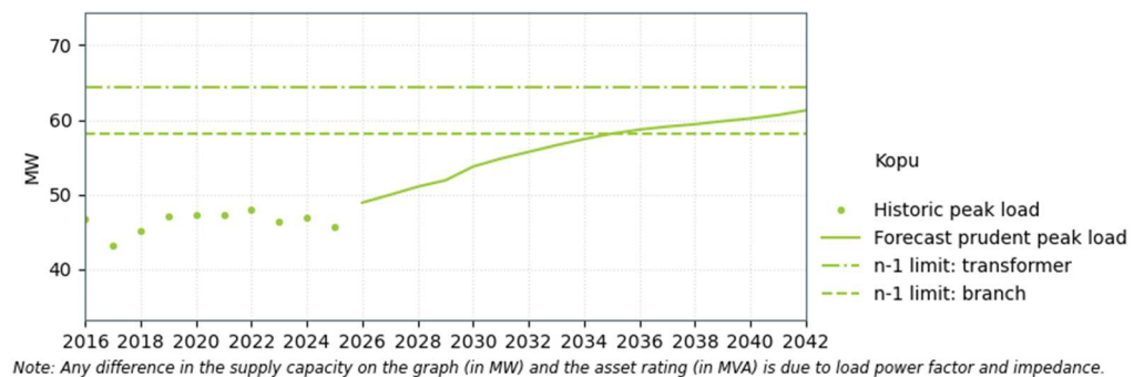
Figure 9-17: Kopu supply capacity
