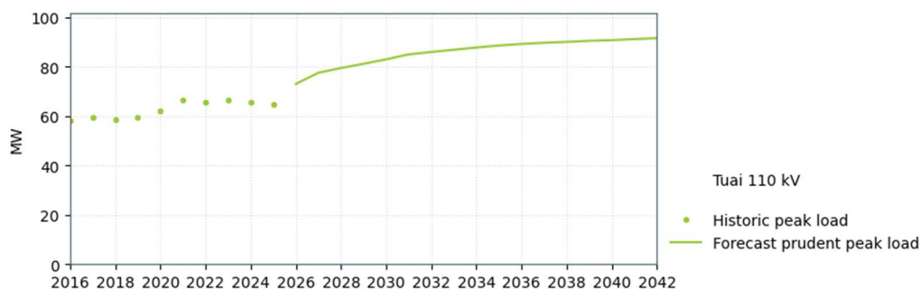
Figure 13-10: Tuai 110 kV load forecast
