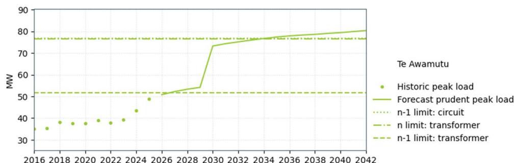
Figure 9-19: Te Awamutu supply capacity
