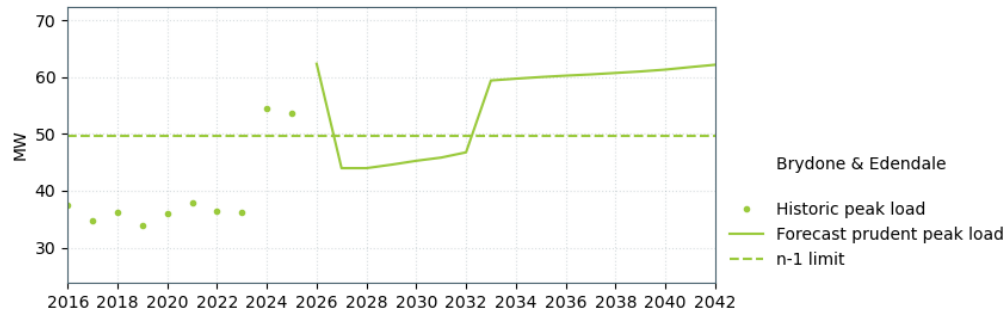
Figure 19-5: Brydone–Gore–1 and Edendale–Invercargill–1 capacity
