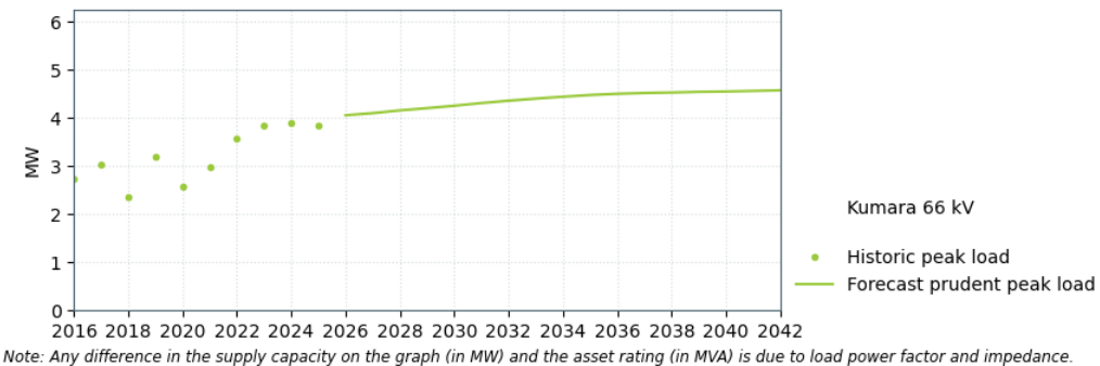
Figure 16-9: Kumara load forecast
