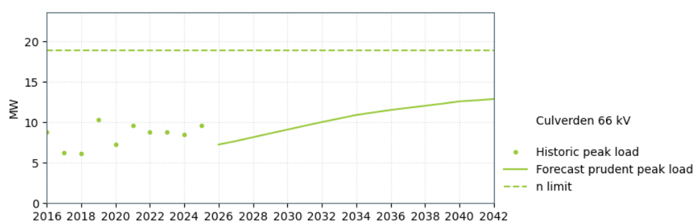
Figure 17-13: Culverden 33/66 kV supply capacity
