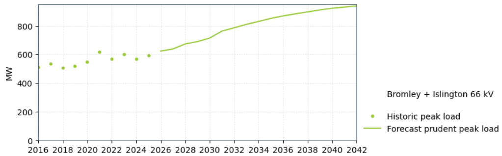
Figure 17-4: Bromley and Islington combined 66 kV load
