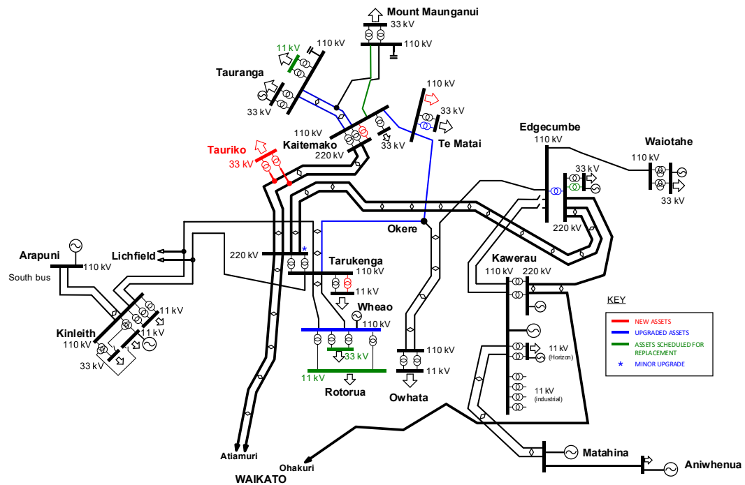
Figure 10-3: Possible Bay of Plenty region transmission configuration in 2041
