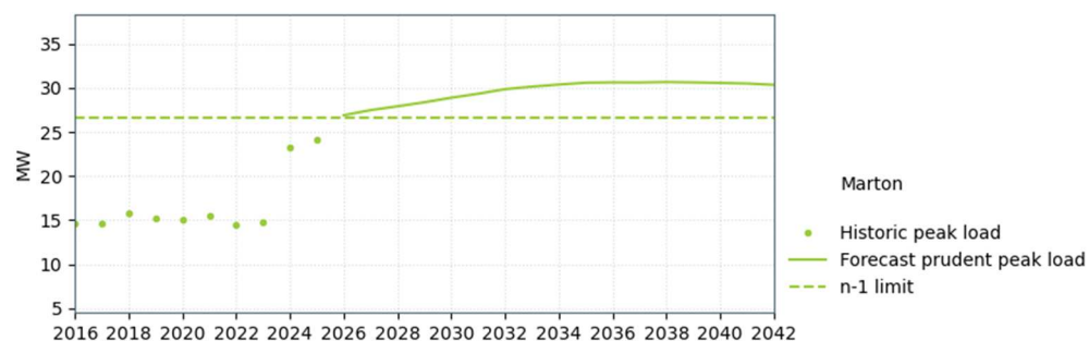
Figure 12-11: Marton Supply Capacity
