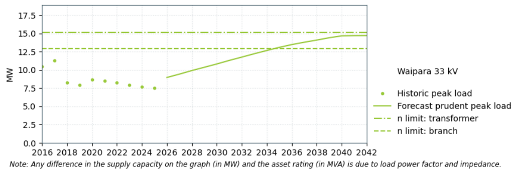
Figure 17-22: Waipara 33 kV supply capacity
