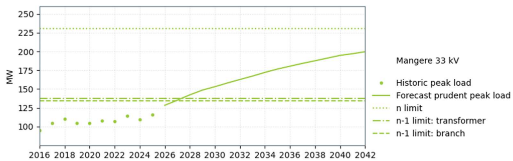
Figure 8-12: Mangere 33 kV supply capacity
