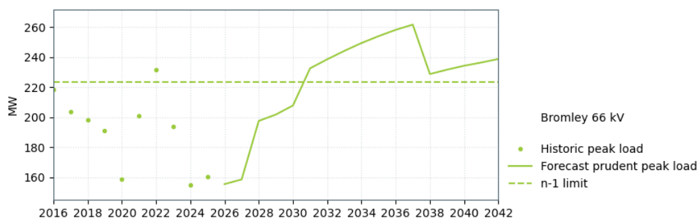
Figure 17-10: Bromley supply capacity
