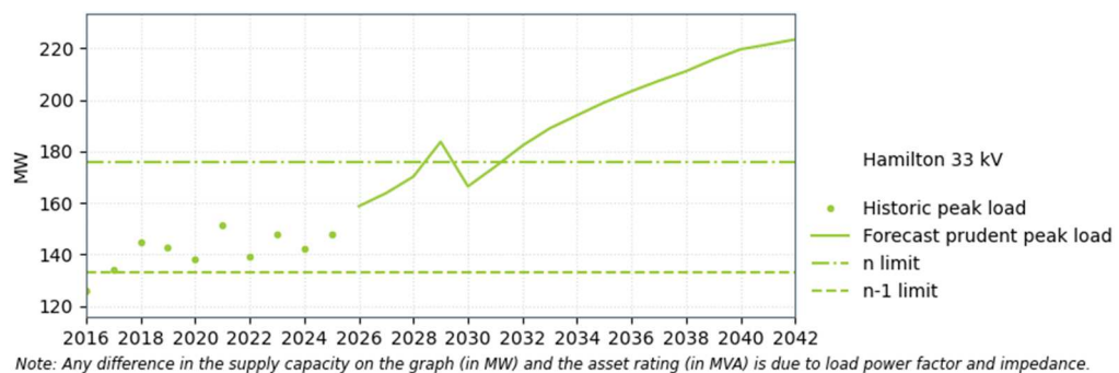
Figure 9-10: Hamilton 33 kV supply capacity
