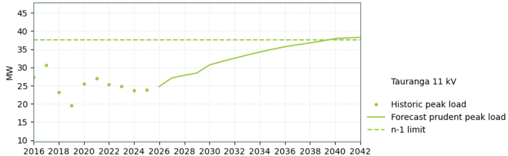
Figure 10-22: Tauranga 110/11 kV supply capacity
