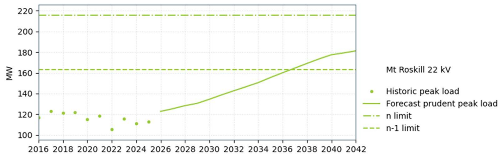
Figure 8-14: Mount Roskill 22 kV supply capacity
