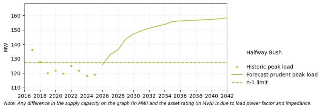
Figure 19-14: Halfway Bush supply capacity
