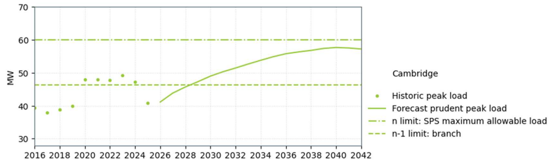
Figure 9-9: Cambridge supply capacity
