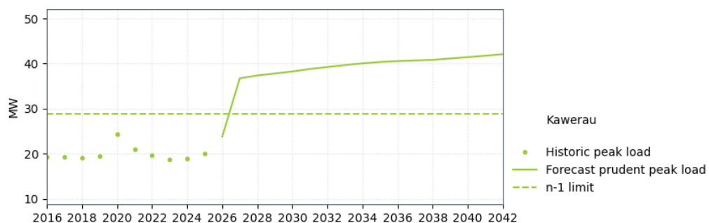
Figure 10-12: Kawerau (Horizon) supply capacity
